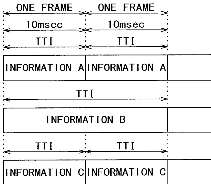
FIG. 9 RELATED ART
