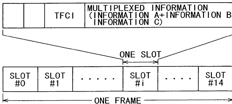
FIG. 10 RELATED ART
