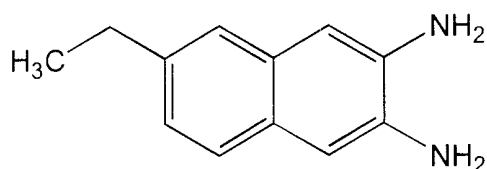
6-Ethyl-2,3-diamino naphthalene
