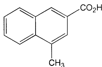
4-Methyl-2-naphthoic acid
