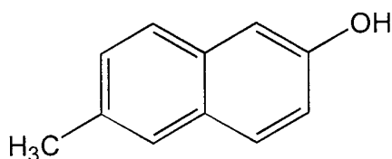
6-Methyl naphth-2-ol
