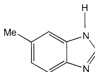
5-Methyl benzimidazole
