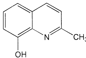
8-hydroxy quinaldine
