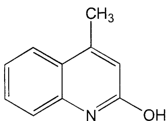
2-hydroxy-4-methyl quinoline
