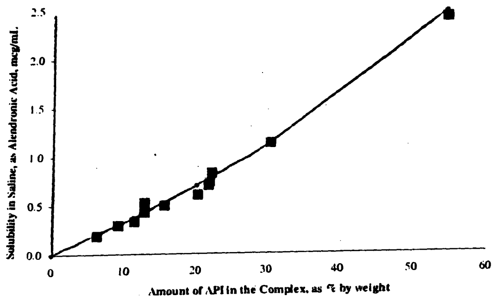
Fig. 1 Solubility of AC-PC vs. Amount of API in the Complex
