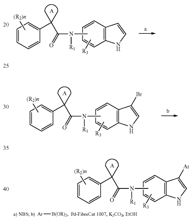
Scheme 37
