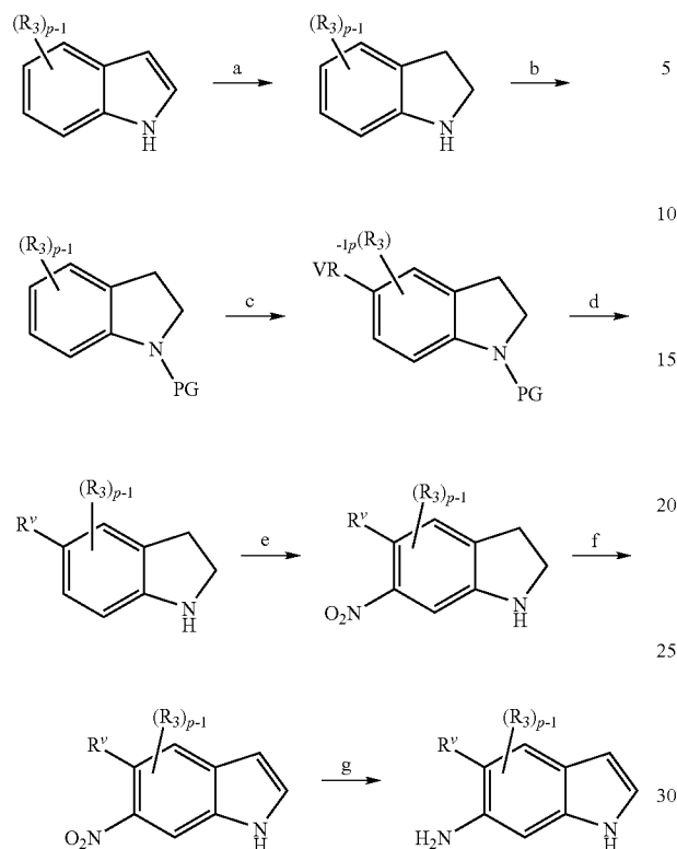
Scheme 14
