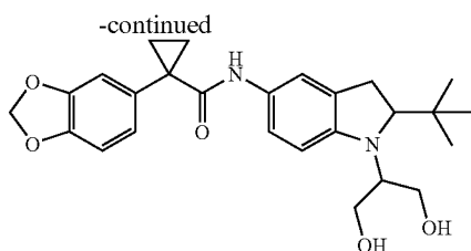
1-(Benzo[d][1,3]dioxol-5-yl)-N-(2-tert-butyl-1-(1,3-dihydroxypropan-2-yl)indolin-5-yl)cyclopropanecarboxamide
