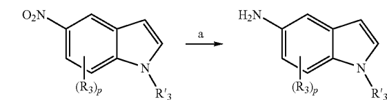
Scheme 24
