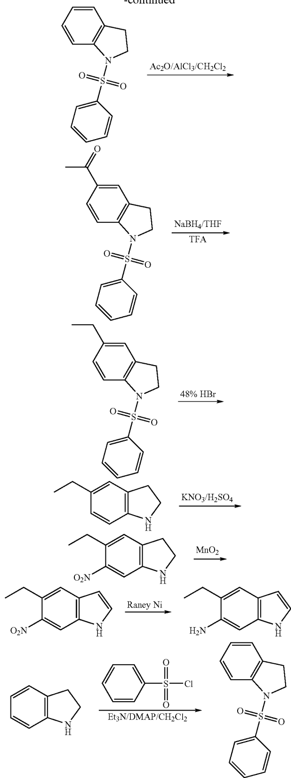
1-(Phenylsulfonyl)indoline
