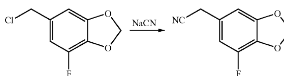
2-(7-Fluorobenzo[d][1,3]dioxol-5-yl)acetonitrile
