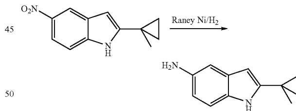
2-(1-Methyl-cyclopropyl)-1H-indol-5-ylamine
