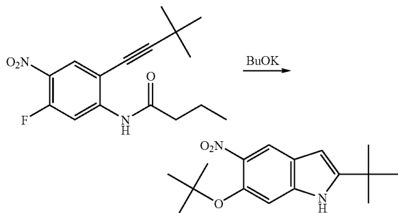
6-tert-Butoxy-2-tert-butyl-5-nitro-1H-indole
