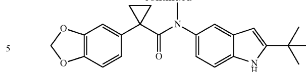
1-(Benzo[d][1,3]dioxol-5-yl)-N-(2-tert-butyl-1H-indol-5-yl)-N-methylcyclopropanecarboxamide
