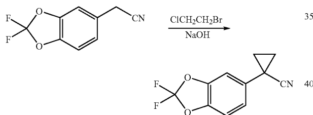
1-(2,2-Difluoro-benzo[1,3]dioxol-5-yl)-cyclopropanecarbonitrile
