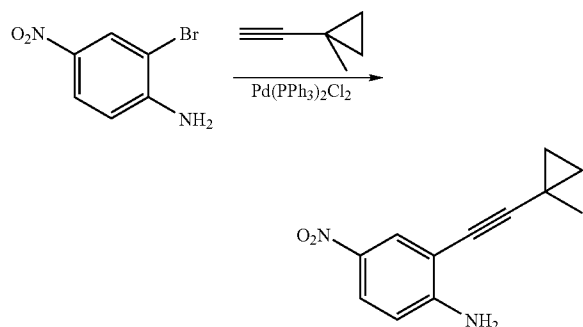
2-((1-Methylcyclopropyl)ethynyl)-4-nitroaniline
