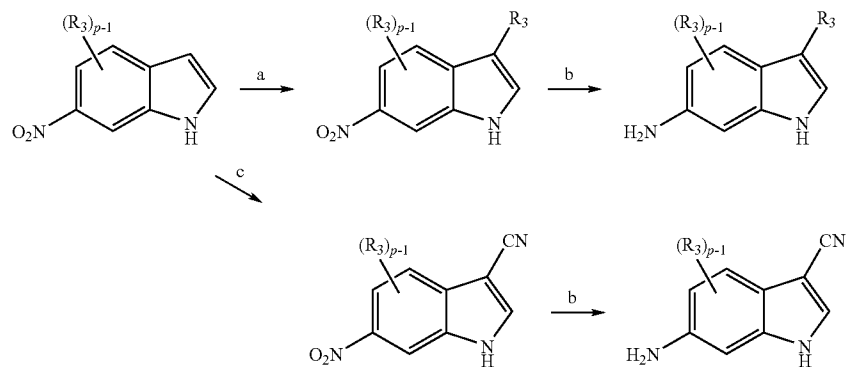
Scheme 15
