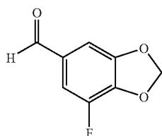
7-Fluoro-benzo[1,3]dioxole-5-carbaldehyde
