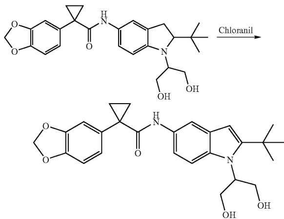
1-(Benzo[d][1,3]dioxol-5-yl)-N-(2-tert-butyl-1-(1,3-dihydroxypropan-2-yl)-1H-indol-5-yl)cyclopropanecarboxamide
