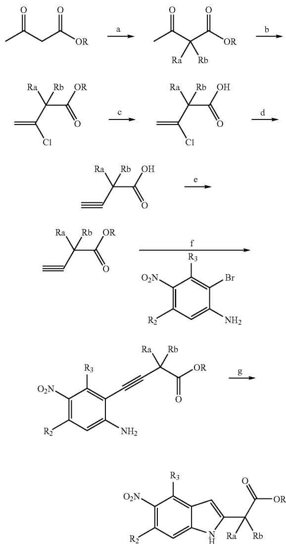
Scheme 42
