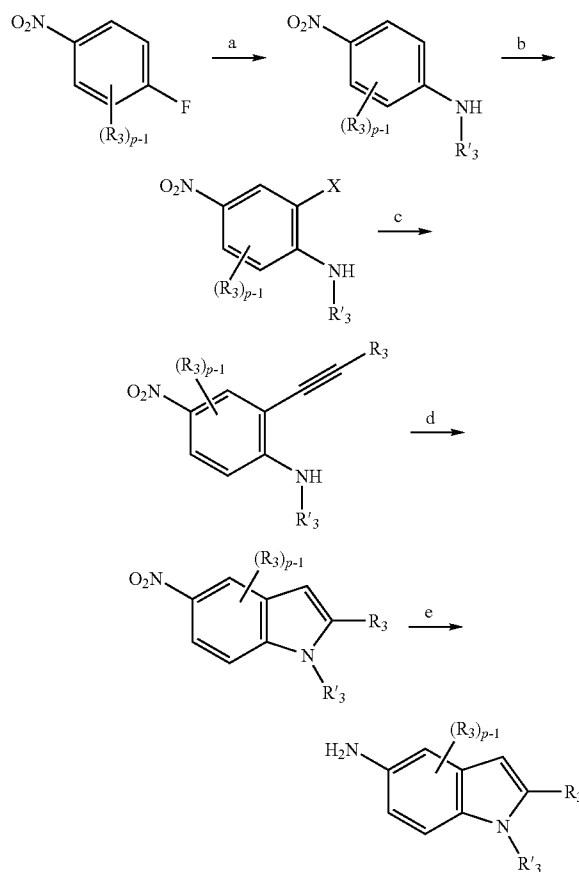
Scheme 20
