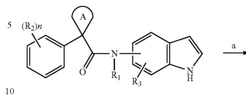
Scheme 34
