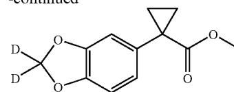
Methyl 1-(2,2-dideuterio-1-(3,4-dihydroxyphenyl)cyclopropanecarboxylate
