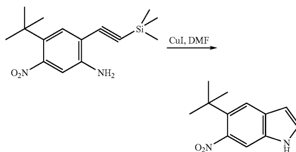
5-tert-Butyl-6-nitro-1H-indole
