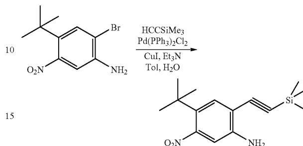
4-tert-Butyl-5-nitro-2-trimethylsilyl-ethynyl-phenylamine
