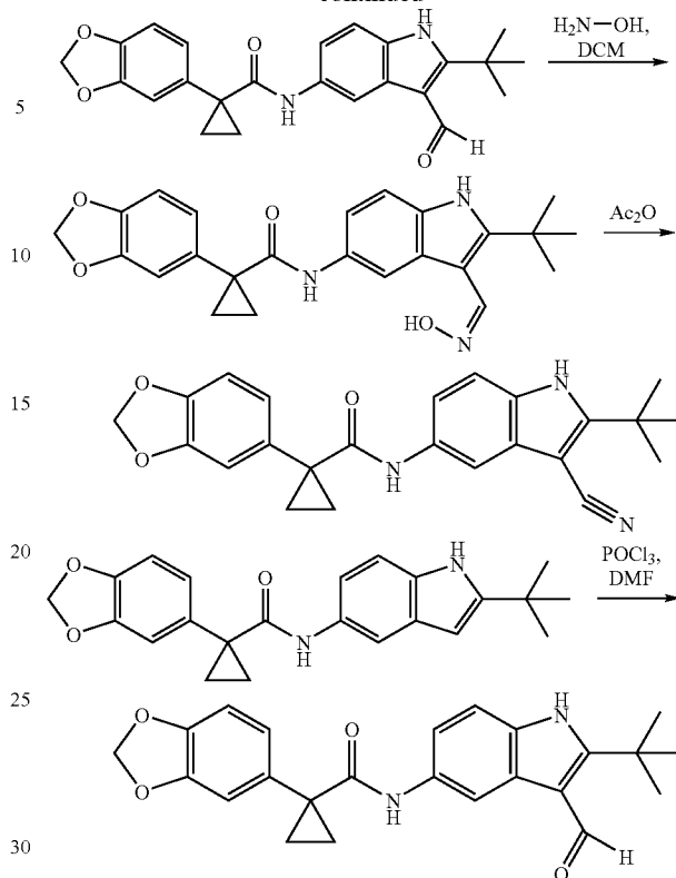
1-(Benzo[d][1,3]dioxol-5-yl)-N-(2-tert-butyl-3-formyl-1H-indol-5-yl)cyclopropanecarboxamide
