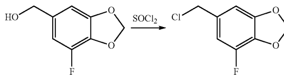
6-Chloromethyl-4-fluoro-benzo[1,3]dioxole
