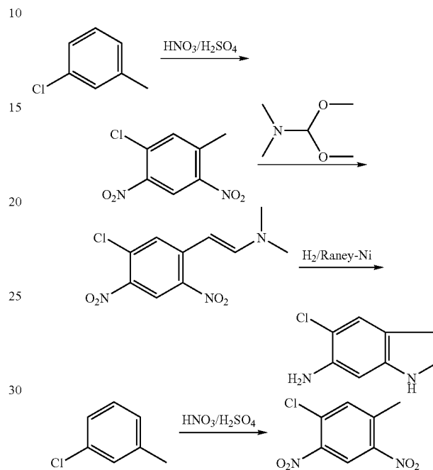
1-Chloro-5-methyl-2,4-dinitrobenzene
