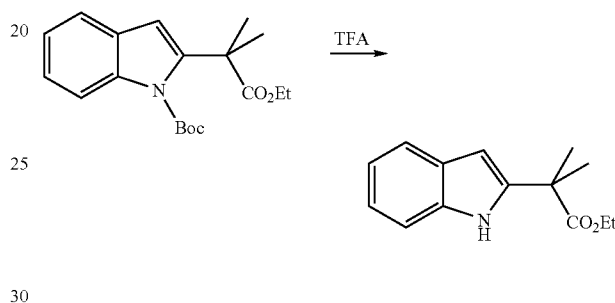
Ethyl 2-(1H-indol-2-yl)-2-methylpropanoate
