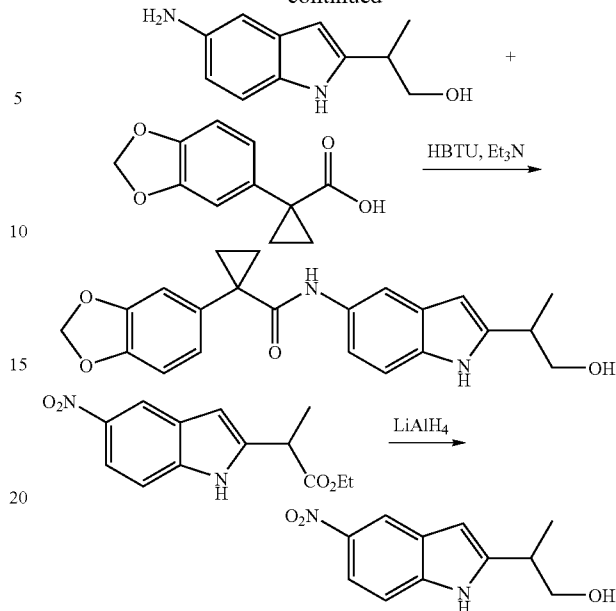
2-(5-Nitro-1H-indol-2-yl)propan-1-ol
