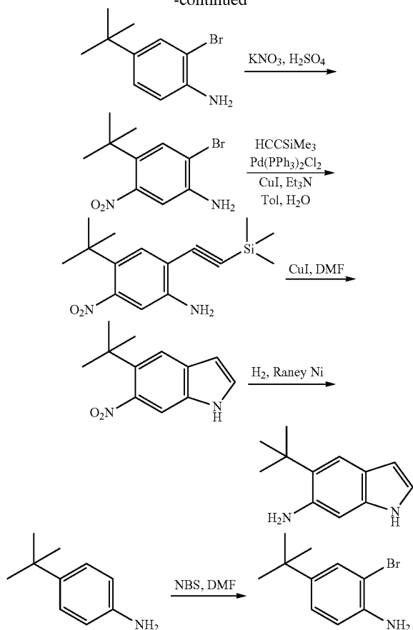
2-Bromo-4-tert-butyl-phenylamine
