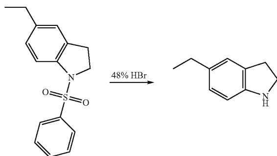
5-Ethylindoline
