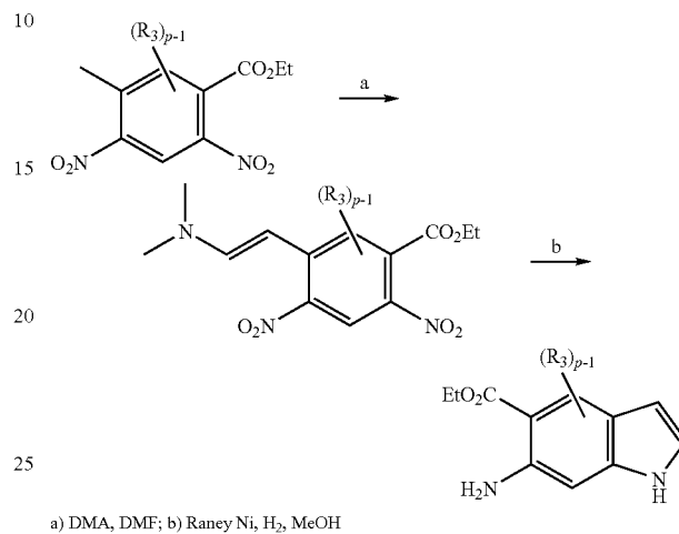
Scheme 11
