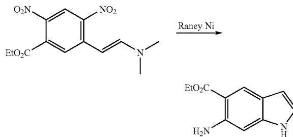
Ethyl 6-amino-1H-indole-5-carboxylate
