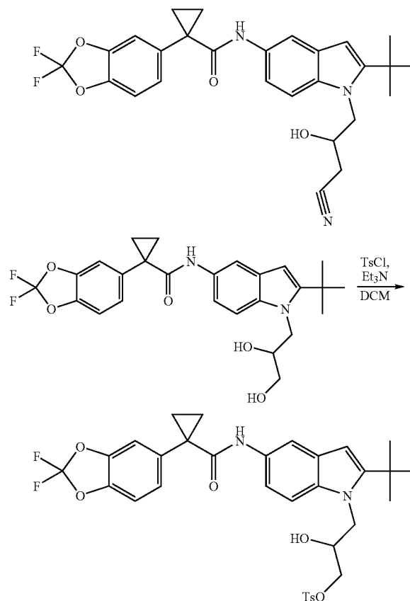
3-(2-tert-Butyl-5-(1-(2,2-difluorobenzo[d][1,3]dioxol-5-yl)cyclopropanecarboxamido)-1H-indol-1-yl)-2-hydroxypropyl-4-methylbenzenesulfonate
