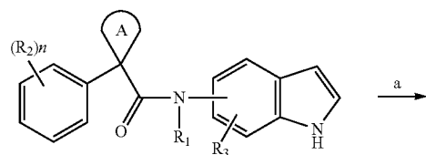
Scheme 36
