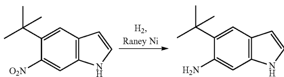
5-tert-Butyl-1H-indol-6-ylamine
