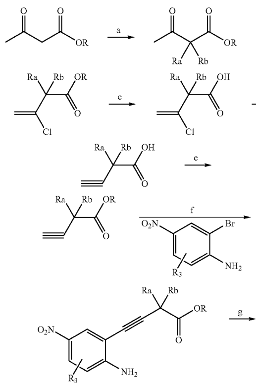
Scheme 31
