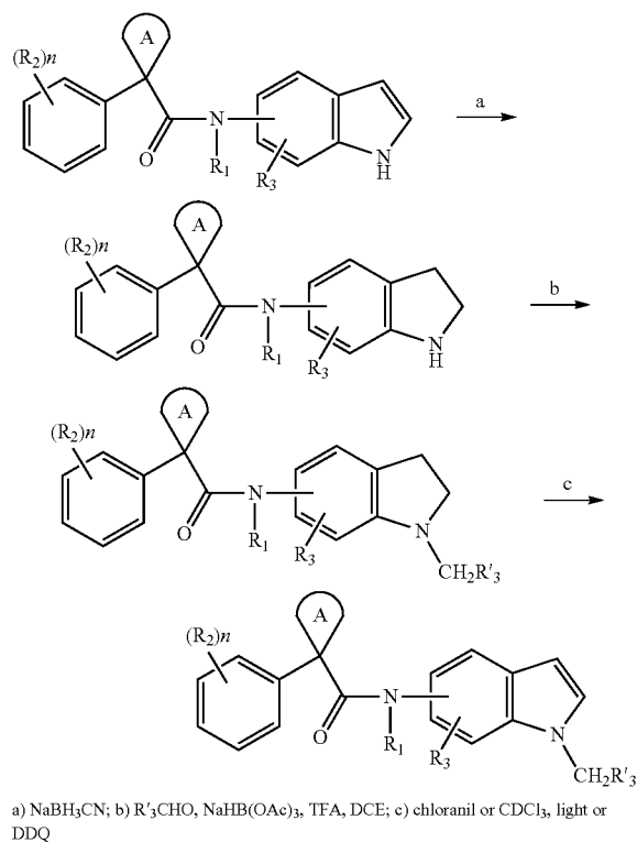
Scheme 35
