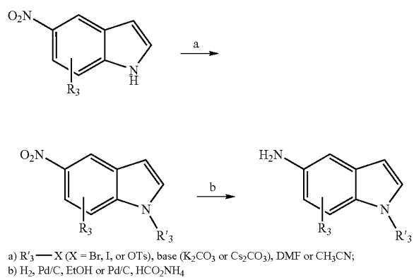
Scheme 27
