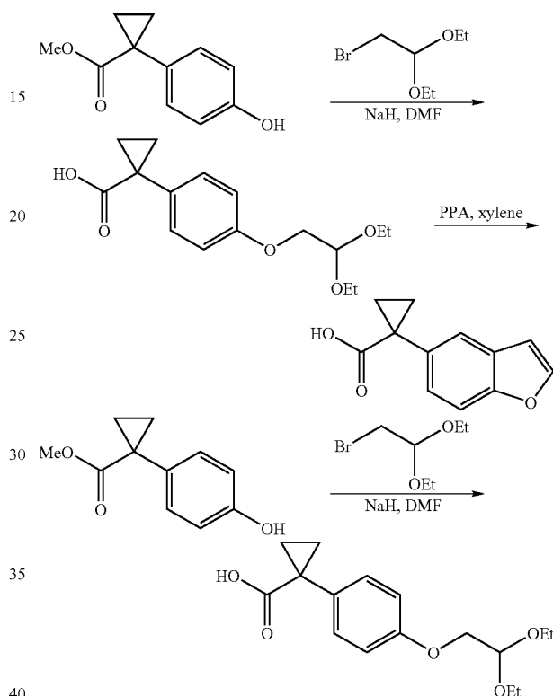
1-[4-(2,2-Diethoxy-ethoxy)-phenyl]-cyclopropanecarboxylic acid
