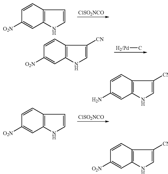
6-Nitro-1H-indole-3-carbonitrile
