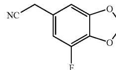
2-(7-Fluorobenzo[d][1,3]dioxol-5-yl)acetonitrile
