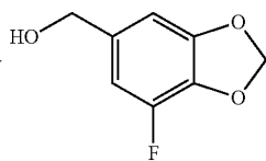
(7-Fluoro-benzo[1,3]dioxol-5-yl)-methanol
