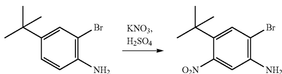
2-Bromo-4-tert-butyl-5-nitro-phenylamine
