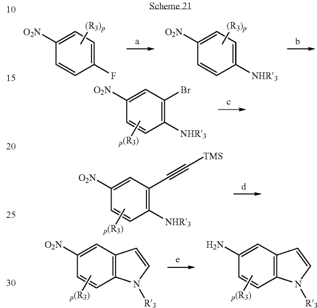
Scheme 21
