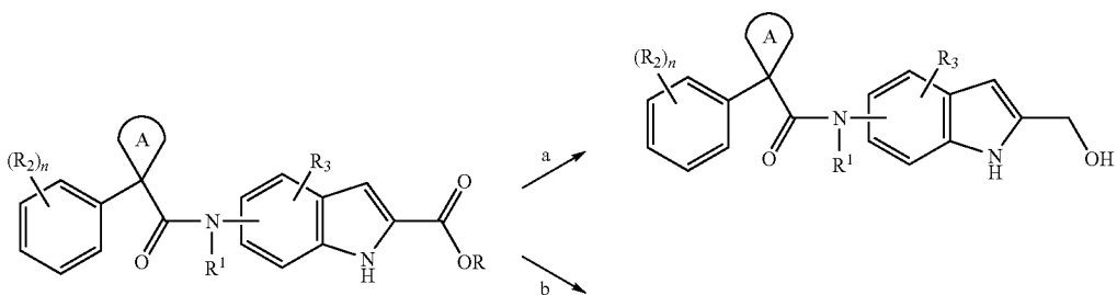
Scheme 33
