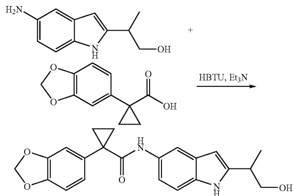
1-(Benzo[d][1,3]dioxol-5-yl)-N-(2-(1-hydroxypropan-2-yl)-1H-indol-5-yl)cyclopropanecarboxamide
