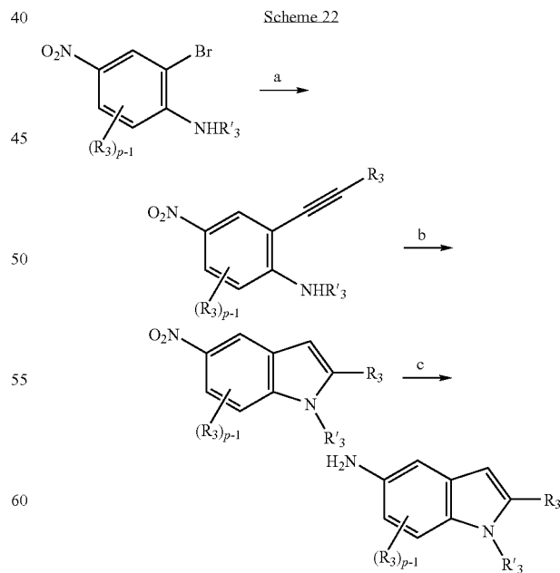
Scheme 22
