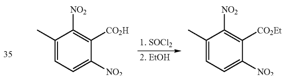
Ethyl 3-methyl-2,6-dinitrobenzoate
