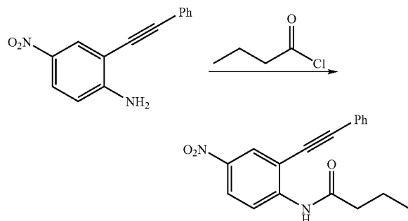
N-(2-(Phenylethynyl)phenyl)-4-nitrobutyramide
