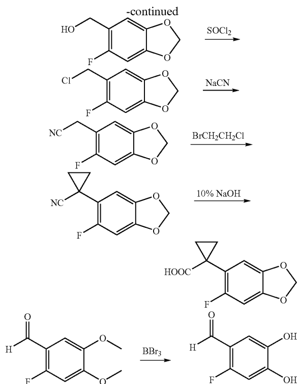
2-Fluoro-4,5-dihydroxy-benzaldehyde
