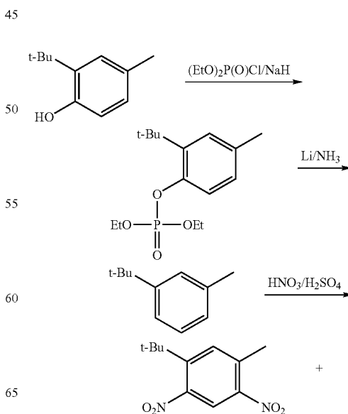
5-tert-Butyl-1H-indol-6-amine
