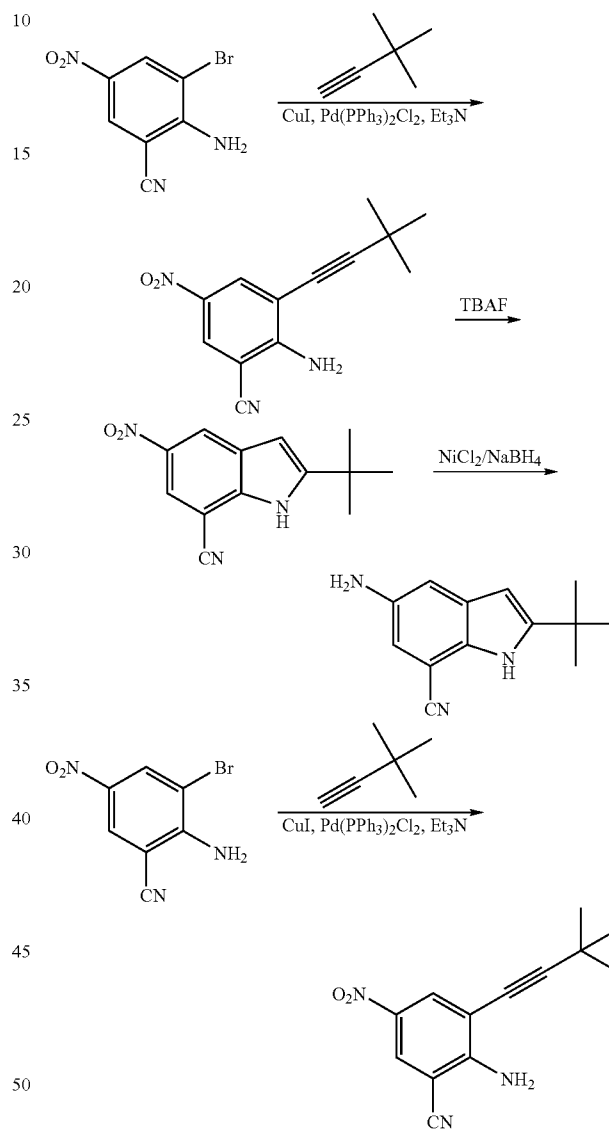
5-Amino-2-tert-butyl-1H-indole-7-carbonitrile
