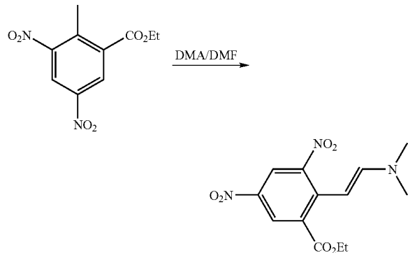
(E)-Ethyl 2-(2-(dimethylamino)vinyl)-3,5-dinitrobenzoate
