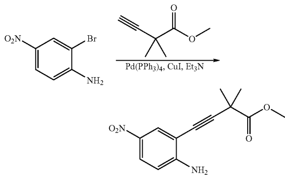
Methyl 4-(2-amino-5-nitrophenyl)-2,2-dimethylbut-3-ynoate
