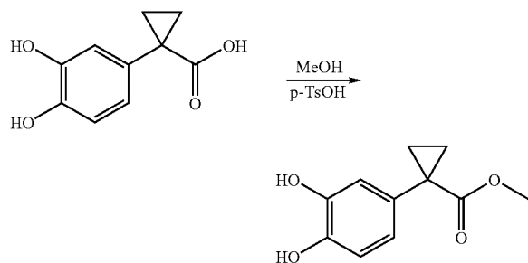
Methyl 1-(3,4-dihydroxyphenyl)cyclopropanecarboxylate
