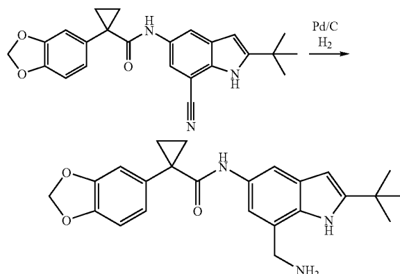
N-(7-(Aminomethyl)-2-tert-butyl-1H-indol-5-yl)-1-(benzo[d][1,3]dioxol-5-yl)cyclopropanecarboxamide
