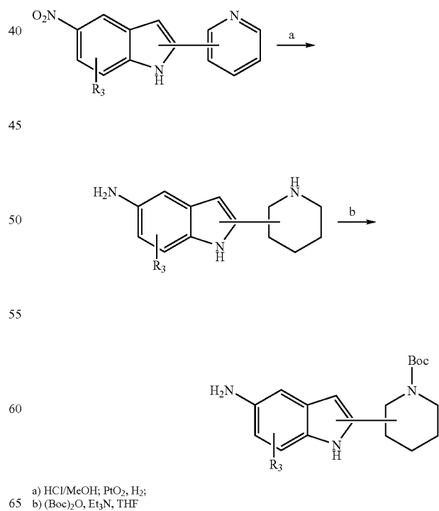
Scheme 29
