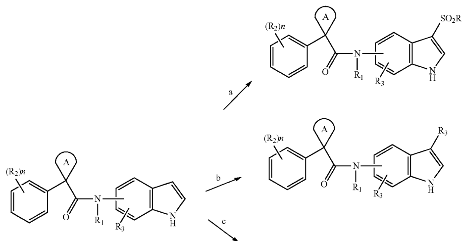
Scheme 38
