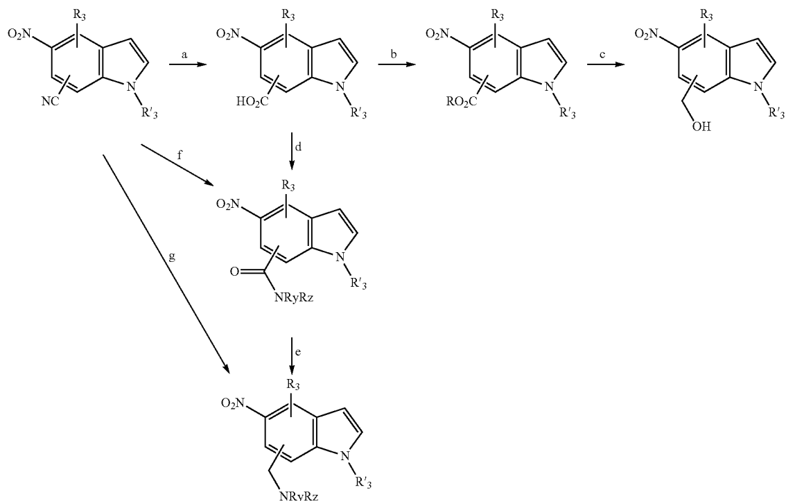
Scheme 30
