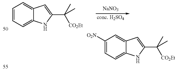
Ethyl 2-methyl-2-(5-nitro-1H-indol-2-yl)propanoate
