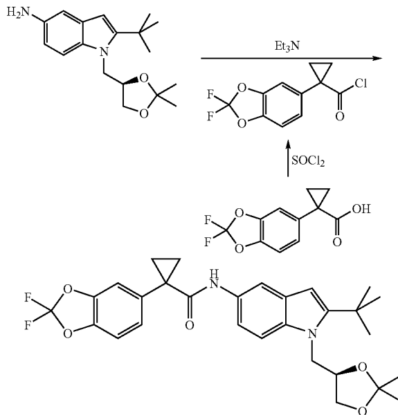
N-((R)-2-tert-Butyl-1-((2,2-dimethyl-1,3-dioxolan-4-yl)methyl)-1H-indol-5-yl)-1-(2,2-difluorobenzo[d][1,3]dioxol-5-yl)cyclopropanecarboxamide
