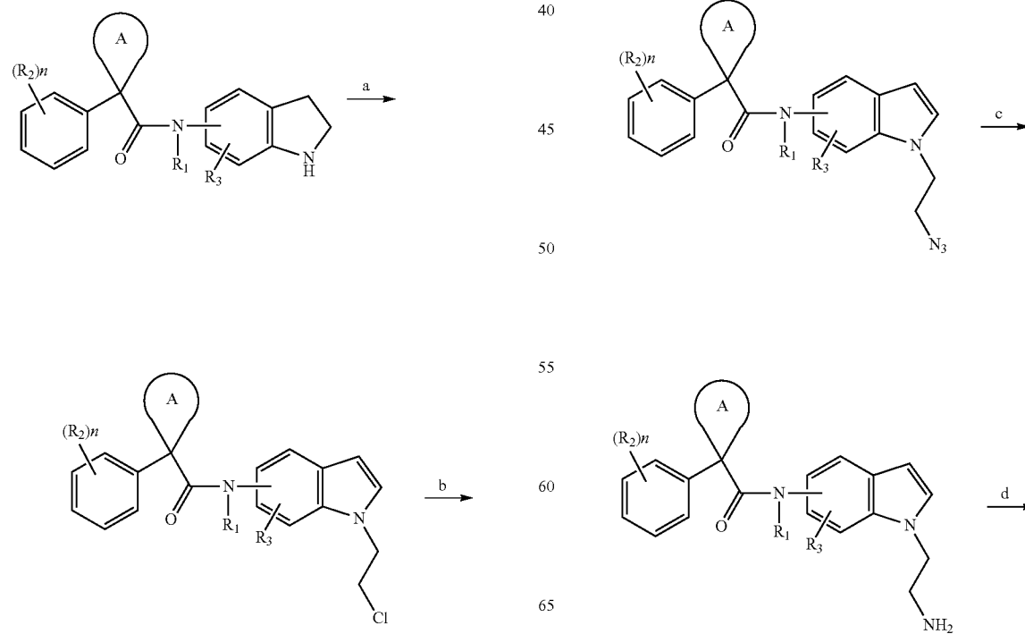
Scheme 41
