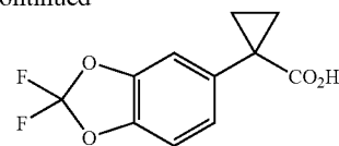
1-(2,2-Difluoro-benzo[1,3]dioxol-5-yl)-cyclopropanecarboxylic acid
