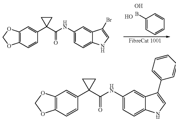
1-(Benzo[d][1,3]dioxol-5-yl)-N-(3-phenyl-1H-indol-5-yl)cyclopropanecarboxamide
