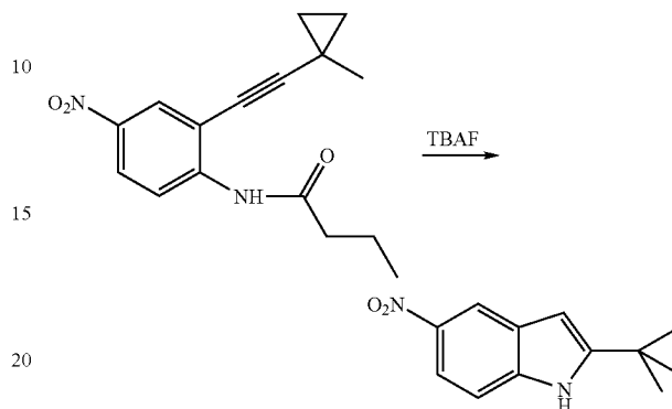
2-(1-Methylcyclopropyl)-5-nitro-1H-indole
