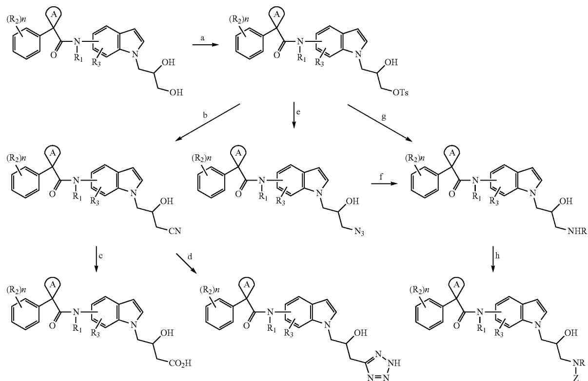
Scheme 40
