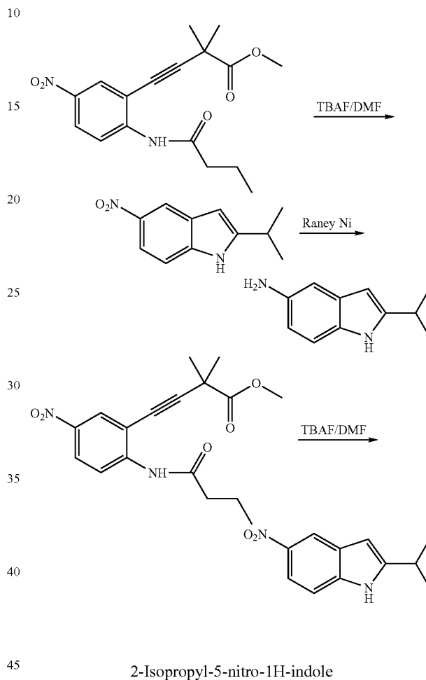
2-Isopropyl-5-nitro-1H-indole
