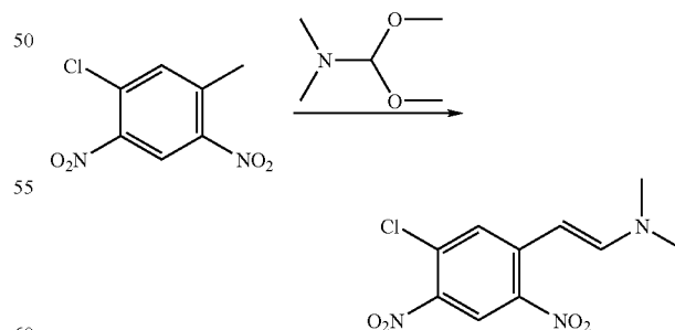
(E)-2-(5-Chloro-2,4-dinitrophenyl)-N,N-dimethylethanamine
