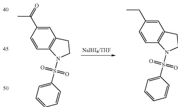
5-Ethyl-1-(phenylsulfonyl)indoline
