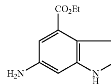
Ethyl 6-amino-1H-indole-4-carboxylate
