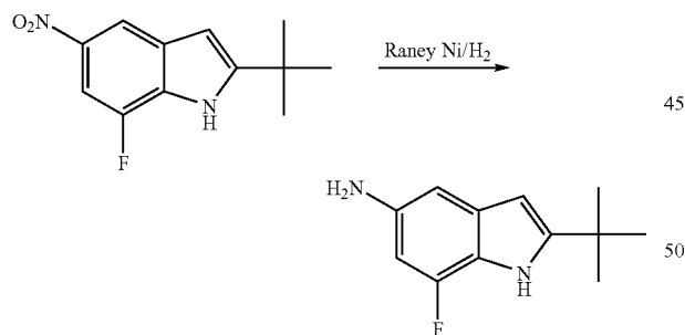
2-tert-Butyl-7-fluoro-1H-indol-5-amine
