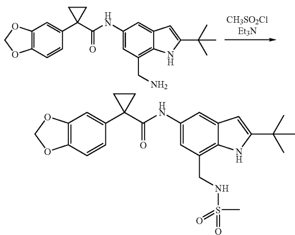
1-(Benzo[d][1,3]dioxol-5-yl)-N-(2-tert-butyl-7-(methylsulfonamidomethyl)-1H-indol-5-yl)cyclopropanecarboxamide
