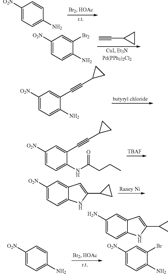
2-Bromo-4-nitroaniline
