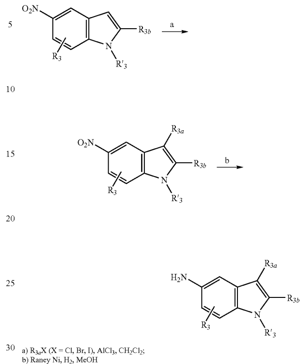
Scheme 28
