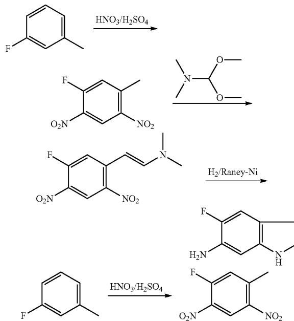
1-Fluoro-5-methyl-2,4-dinitrobenzene
