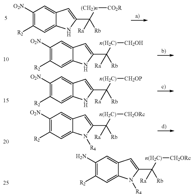
Scheme 43
