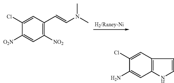
5-Chloro-1H-indol-6-amine
