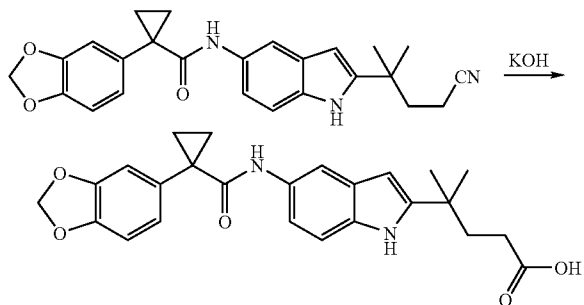
4-(5-(1-(Benzo[d][1,3]dioxol-5-yl)cyclopropanecarboxamido)-1H-indol-2-yl)-4-methylpentanoic acid
