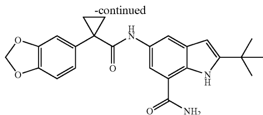
5-(1-(Benzo[d][1,3]dioxol-5-yl)cyclopropanecarboxamido)-2-tert-butyl-1H-indole-7-carboxamide
