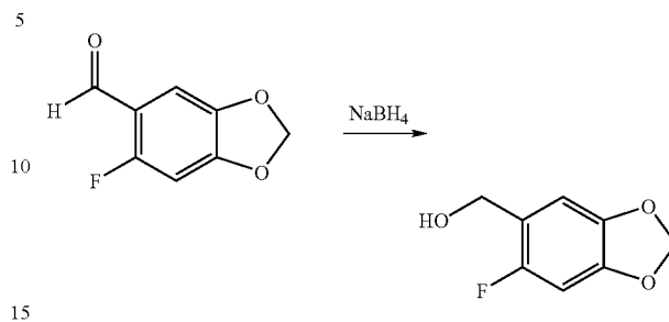
(6-Fluoro-benzo[1,3]dioxol-5-yl)-methanol
