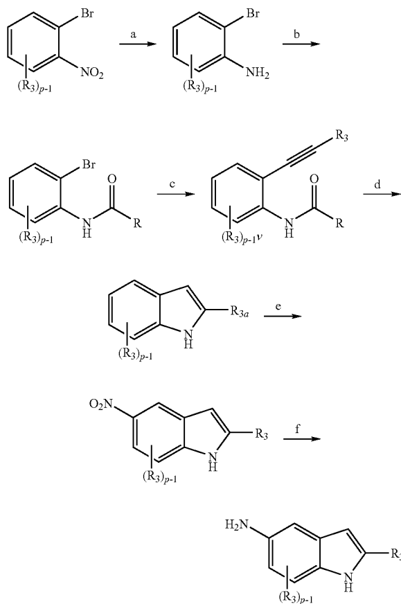
Scheme 23
