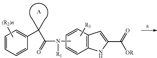
Scheme 32
