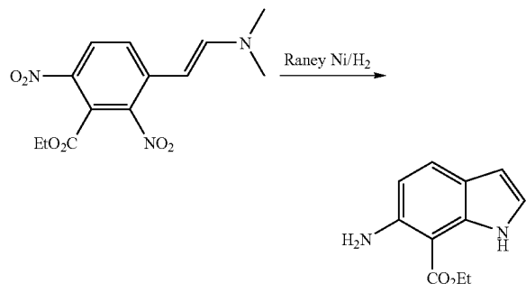
Ethyl 6-amino-1H-indole-7-carboxylate
