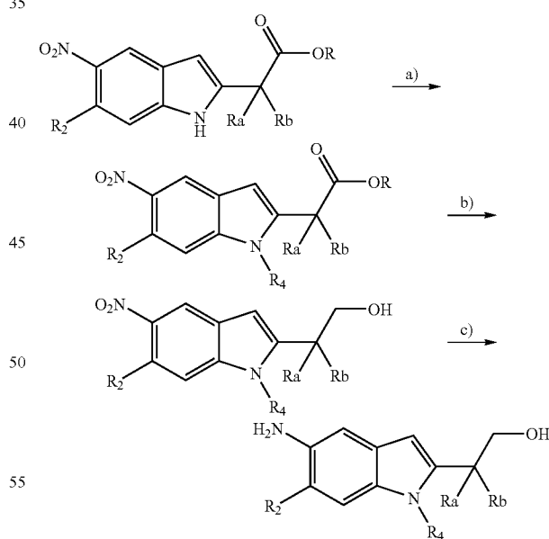
Scheme 43
