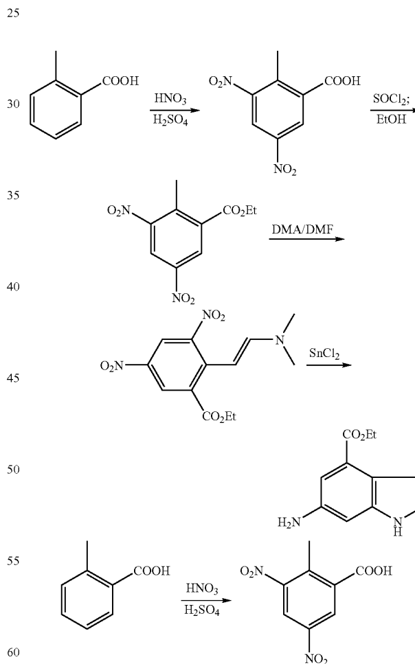
Ethyl 6-amino-1H-indole-4-carboxylate
