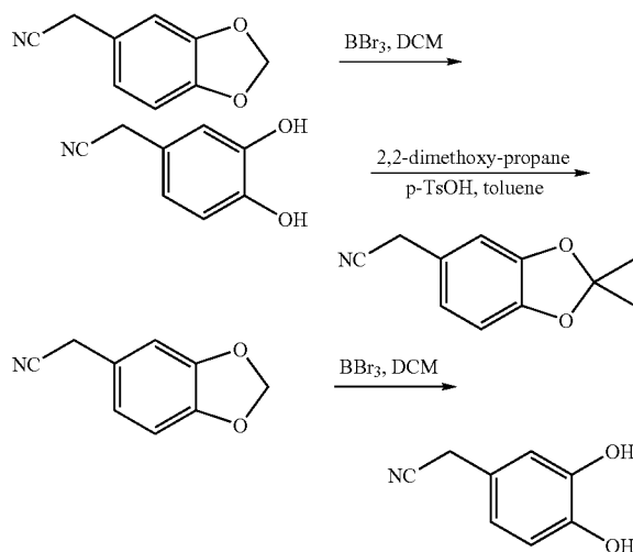
(3,4-Dihydroxy-phenyl)-acetonitrile
