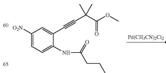
Methyl 4-(2-amino-5-nitrophenyl)-2,2-dimethylbut-3-ynoate
