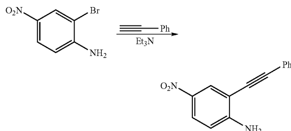
4-Nitro-2-(phenylethynyl)aniline
