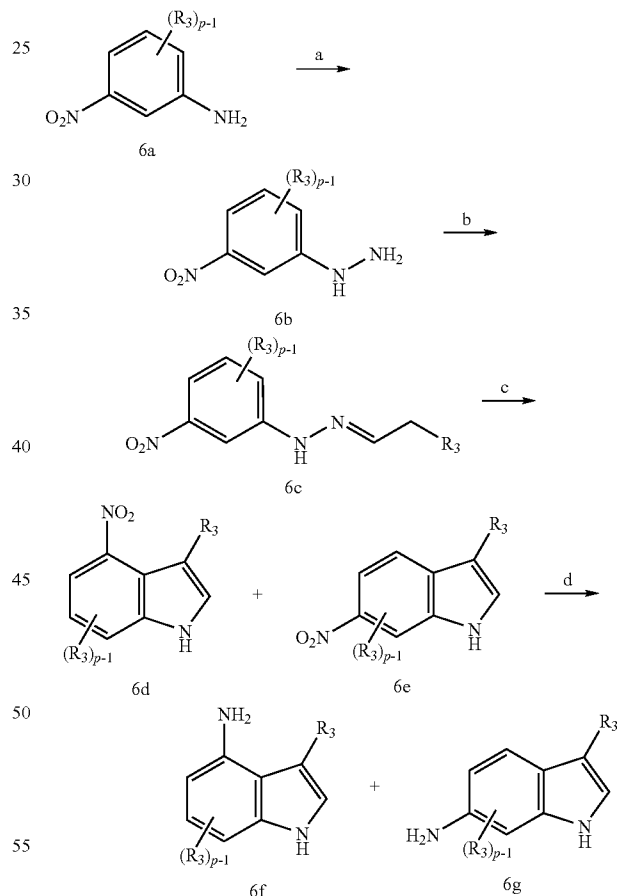
Scheme 6
