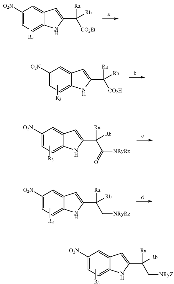
Scheme 26
