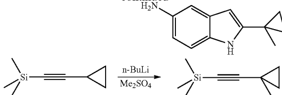
Trimethyl-(1-methyl-cyclopropylethynyl)-silane
