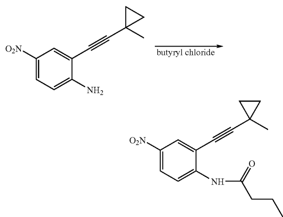
N-[2-(1-Methyl-cyclopropylethynyl)-4-nitro-phenyl]-butyramide
