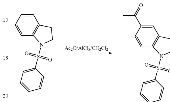
1-(1-(Phenylsulfonyl)indolin-5-yl)ethanone
