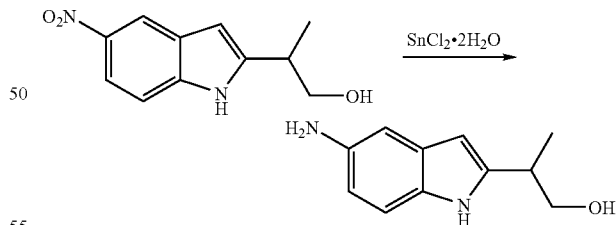
2-(5-Amino-1H-indol-2-yl)propan-1-ol
