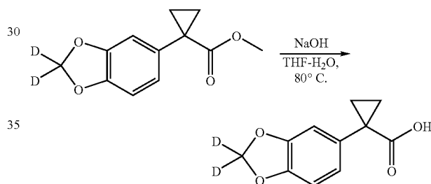
1-(2,2-Dideuterio-1-(3,4-dihydroxyphenyl)cyclopropanecarboxylic acid
