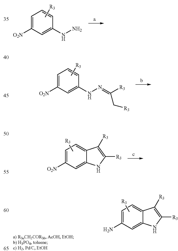
Scheme 12
