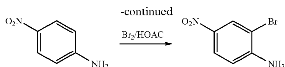
2-Bromo-4-nitroaniline
