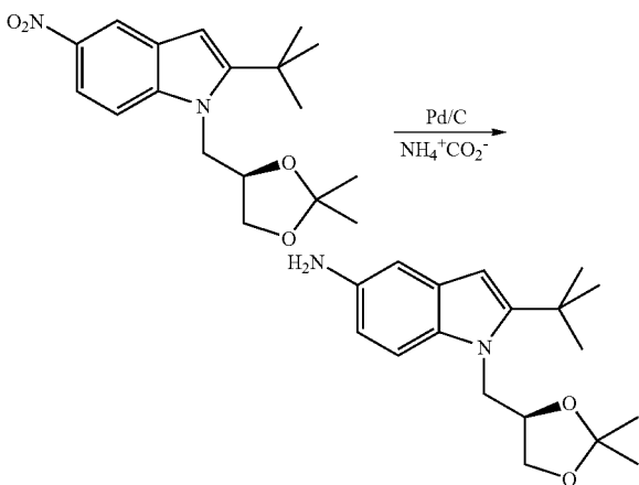
(R)-2-tert-Butyl-1-((2,2-dimethyl-1,3-dioxolan-4-yl)methyl)-1H-indol-5-amine
