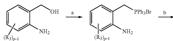
Scheme 25
