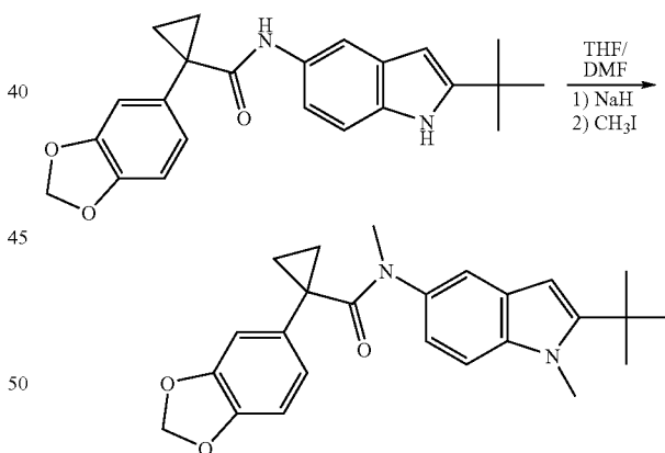
1-(Benzo[d][1,3]dioxol-5-yl)-N-(2-tert-butyl-1H-indol-5-yl)-N-methylcyclopropanecarboxamide
