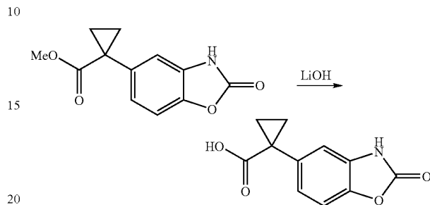
1-(2-Oxo-2,3-dihydrobenzo[d]oxazol-5-yl)cyclopropanecarboxylic acid
