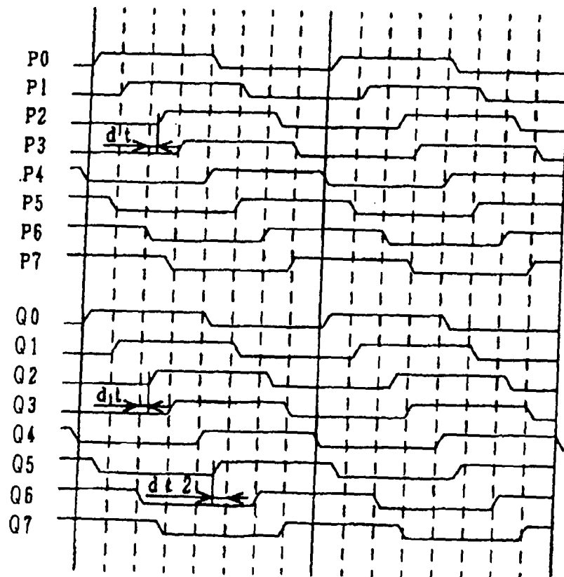
FIG. 17 (b) PRIOR ART
