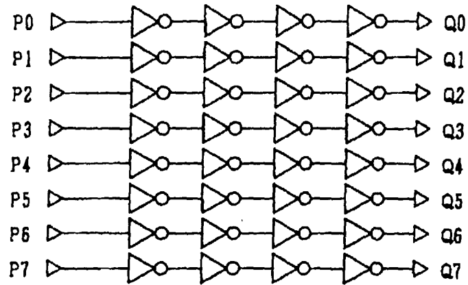
FIG. 17 (a) PRIOR ART
