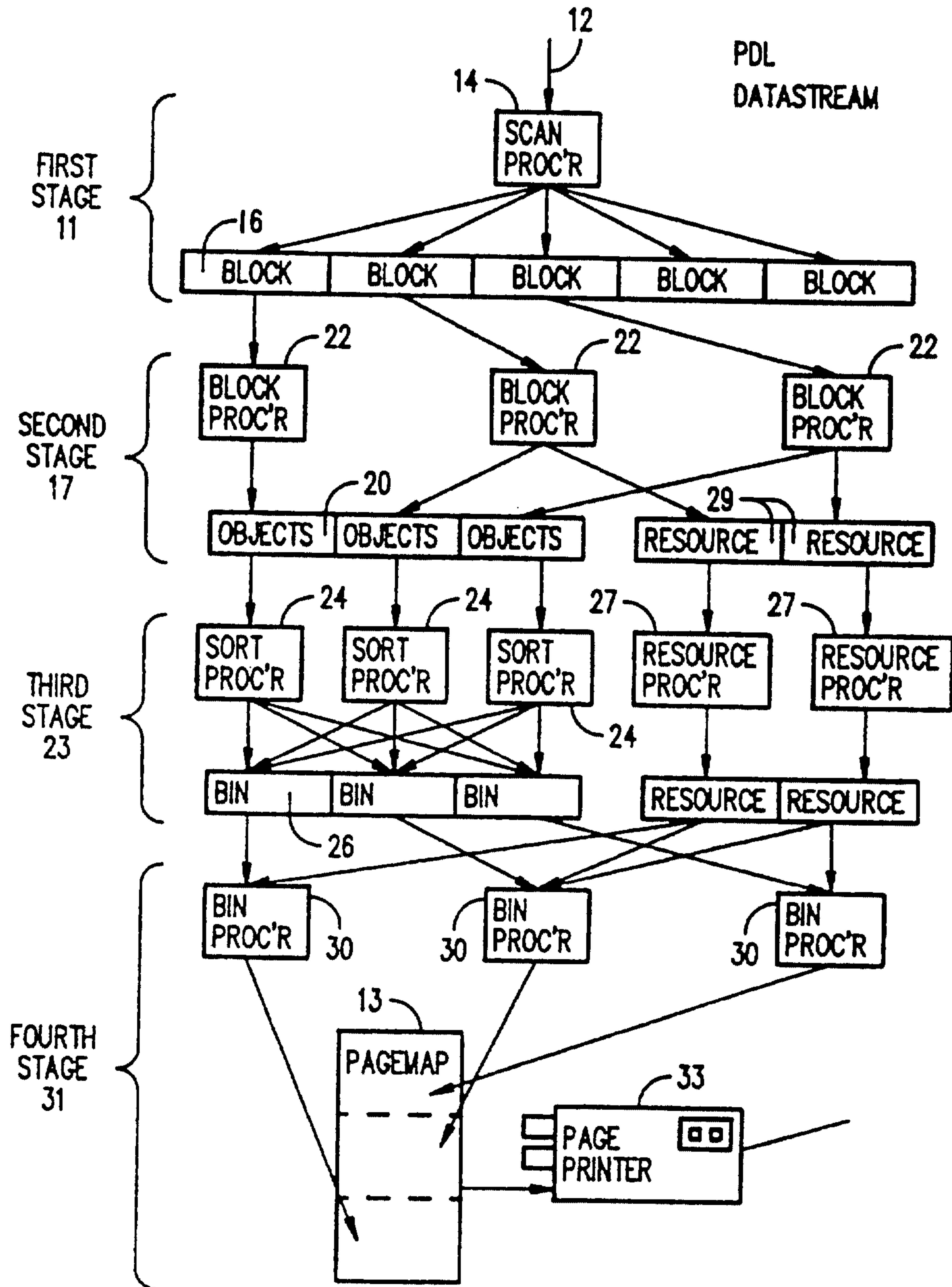
SCHEMATIC FLOWCHART
