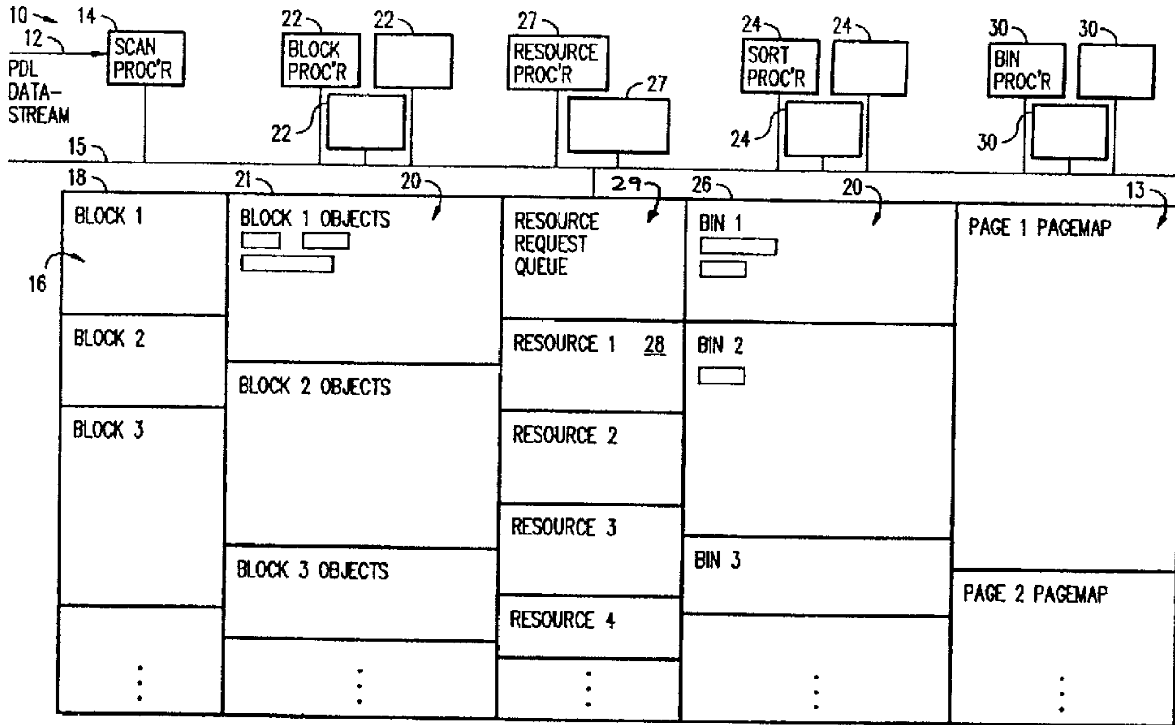
BLOCK DIAGRAM
