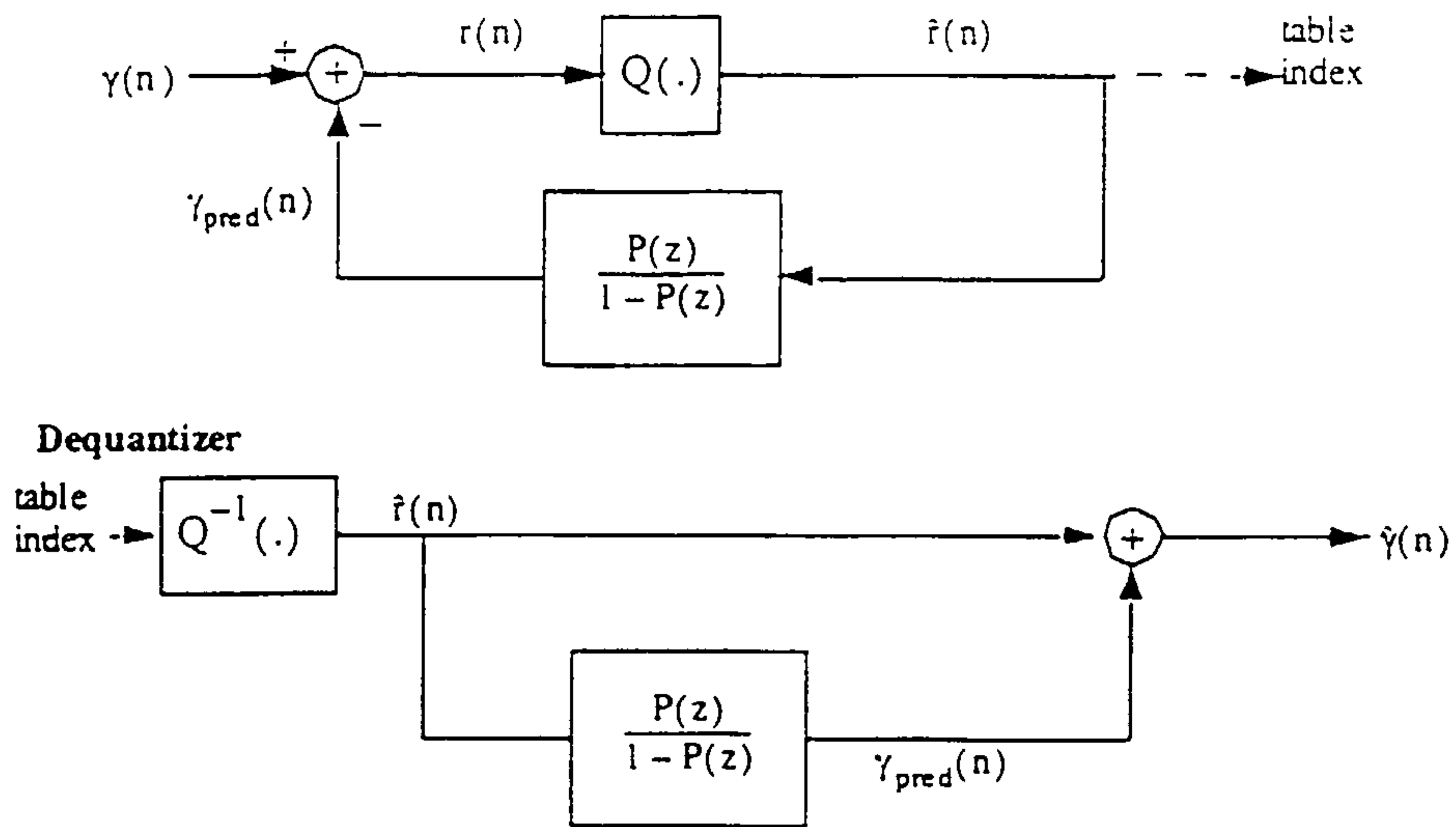
Figure 8 Quantizer
