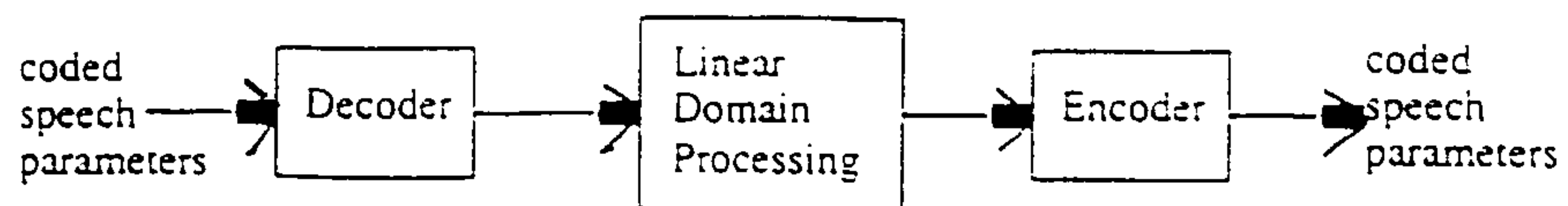
Figure 1: Network enhancement of coded speech in the linear domain
