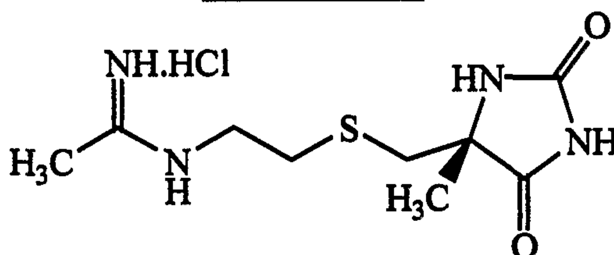
[2-[[[(4R)-4-methyl-2,5-dioxo-4-imidazolidinyl]methyl]thio]ethyl](1-N-iminoethyl)amine
