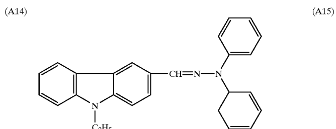
ECH
