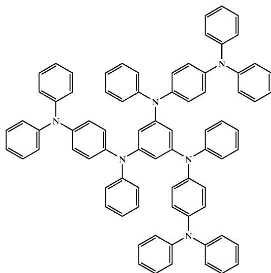
p-DPA-TDAB (T g = 108° C.)
