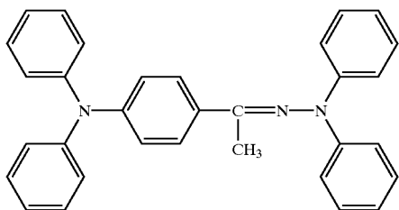
M-DPH
