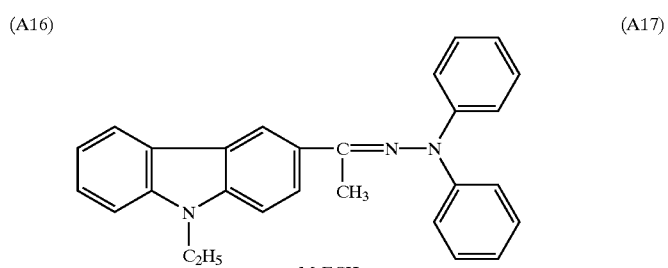
M-ECH
