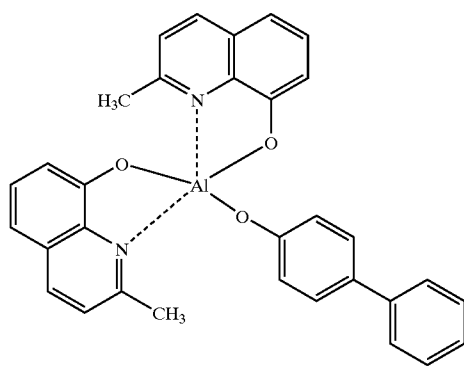
BA1q 2
