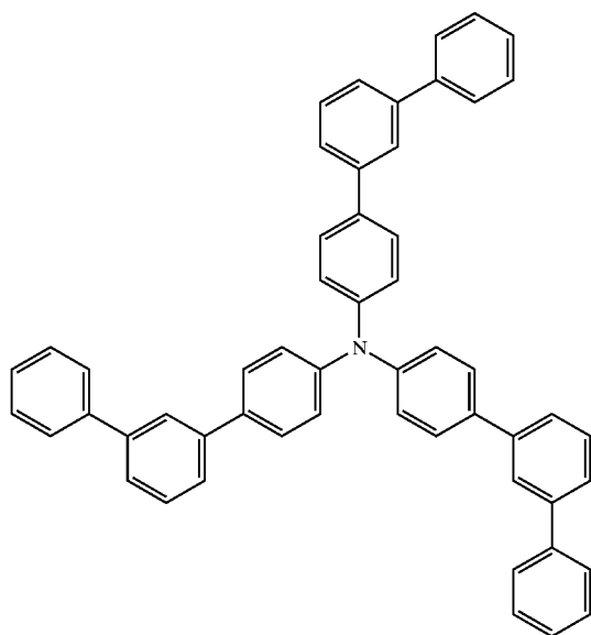
m-TTA
