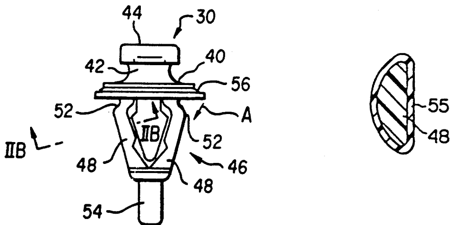
FIG. 2(A) FIG. 2(B)
