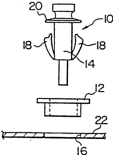
PRIOR ART FIG. 13
