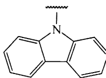
carbazoyl
