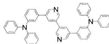
5,5'-bis(3-diphenylaminophenyl)-3,3'-bipyridine
