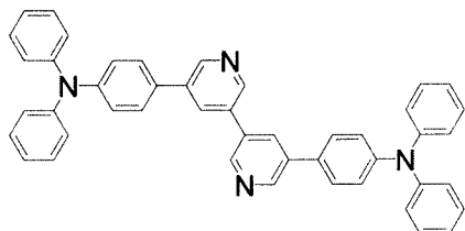
5,5'-bis(4-diphenylaminophenyl)-3,3'-bipyridine
