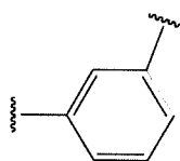
1,3-interphenylene
