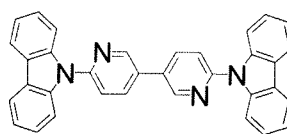
carbazoyl
