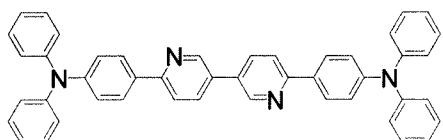
4,4'-(3,3'-bipyridine-6,6'-diyl)bis(N,N-diphenylaniline)
