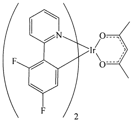
bis(2-[4,6-difluorophenyl]pyridinato-N,C2')iridium(acetylacetonate) [FIr(acac)]
