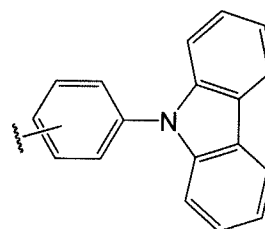
carbazoylphenyl
