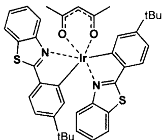
(t-bt) 2 Ir(III)(acac) Bis[2-(4-tert-butylphenyl)benzothiazolato-N,C2'] iridium(III)(acetylacetonate)
