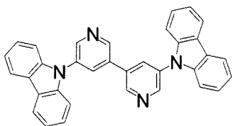
5,5'-(dicarbazole-9-yl)-3,3'-bipyridine
