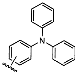
diphenylaminophenyl
