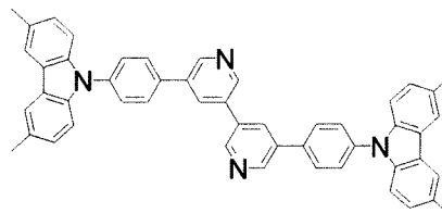
5,5'-bis(4-(3,6-dimethylcarbazol-9-yl)phenyl)-3,3'-bipyridine
