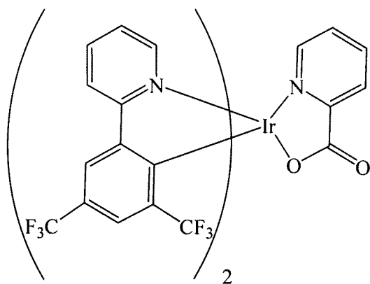
bis-{2-[3,5-bis(trifluoromethyl)phenyl]pyridinato-N,C2'}iridium(III)-picolinate (Ir(CF 3 ppy) 2 (Pic))
