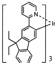
[Ir(Flpy) 3 ] Tris[2-(9,9-dimethylfluoren-2-yl)pyridinato-N,C3'] iridium(III)
