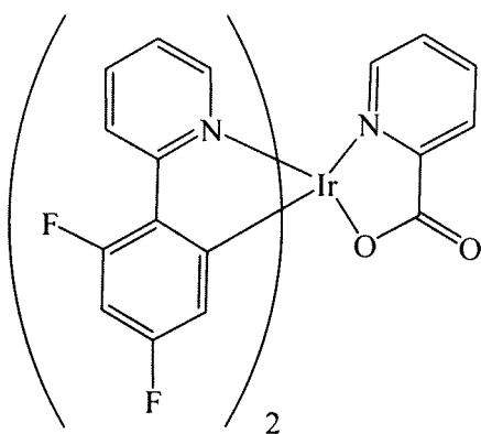
bis(2-[4,6-difluorophenyl]pyridinato-N,C2')iridium (III) picolinate [FIrPic]
