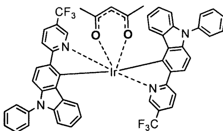
(Cz-CF 3 )Ir(III)(acac) Bis[5-trifluoromethyl-2-[3-(N-phenylcarbazolyl)pyridinato-N,C2'] iridium(III)(acetylacetonate)
