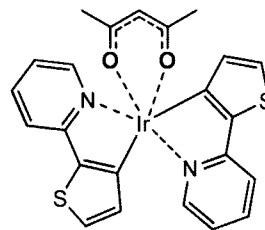
(thp) 2 Ir(III)(acac) Bis[2-(2'-thienyl)pyridinato-N,C3'] iridium(III)(acetylacetonate)
