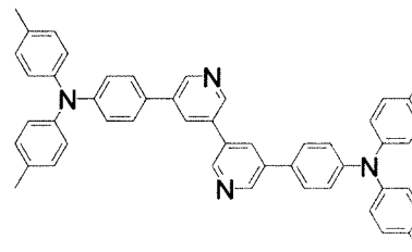
5,5'-bis(4-di(4-methylphenyl)aminophenyl)-3,3'-bipyridine
