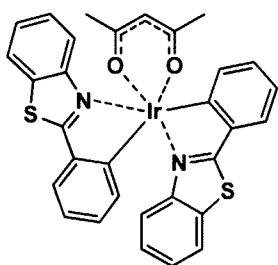
(bt) 2 Ir(III)(acac) Bis[2-phenylbenzothiazolato-N,C2'] iridium(III)(acetylacetonate)
