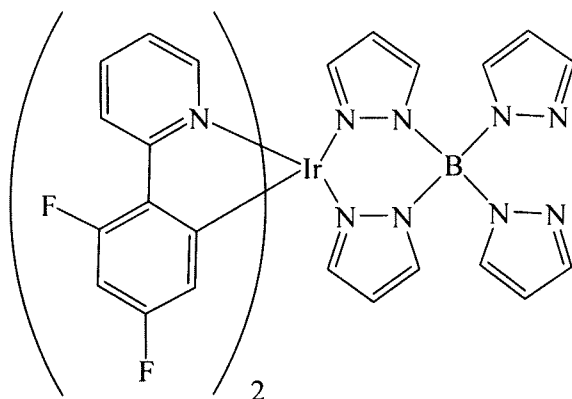
bis[2-(4,6-difluorophenyl)pyridinato-N,C 2' ]iridium(III)tetra(1-pyrazolyl)borate (Fir6)
