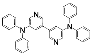
5,5'-bis(diphenylamino)-3,3'- bipyridine
