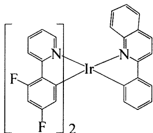
\text{Ir}(\text{dfppy})_2(\text{pq})
