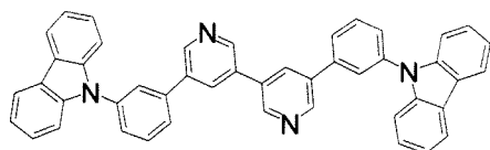
5,5'-bis(3-(carbazol-9-yl)phenyl)-3,3'- bipyridine
