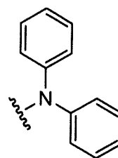
Diphenylamine
