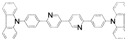
6,6'-bis(4-(carbazol-9-yl)phenyl)-3,3'- bipyridine
