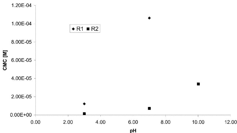
R1/R2 CMC vs. pH
