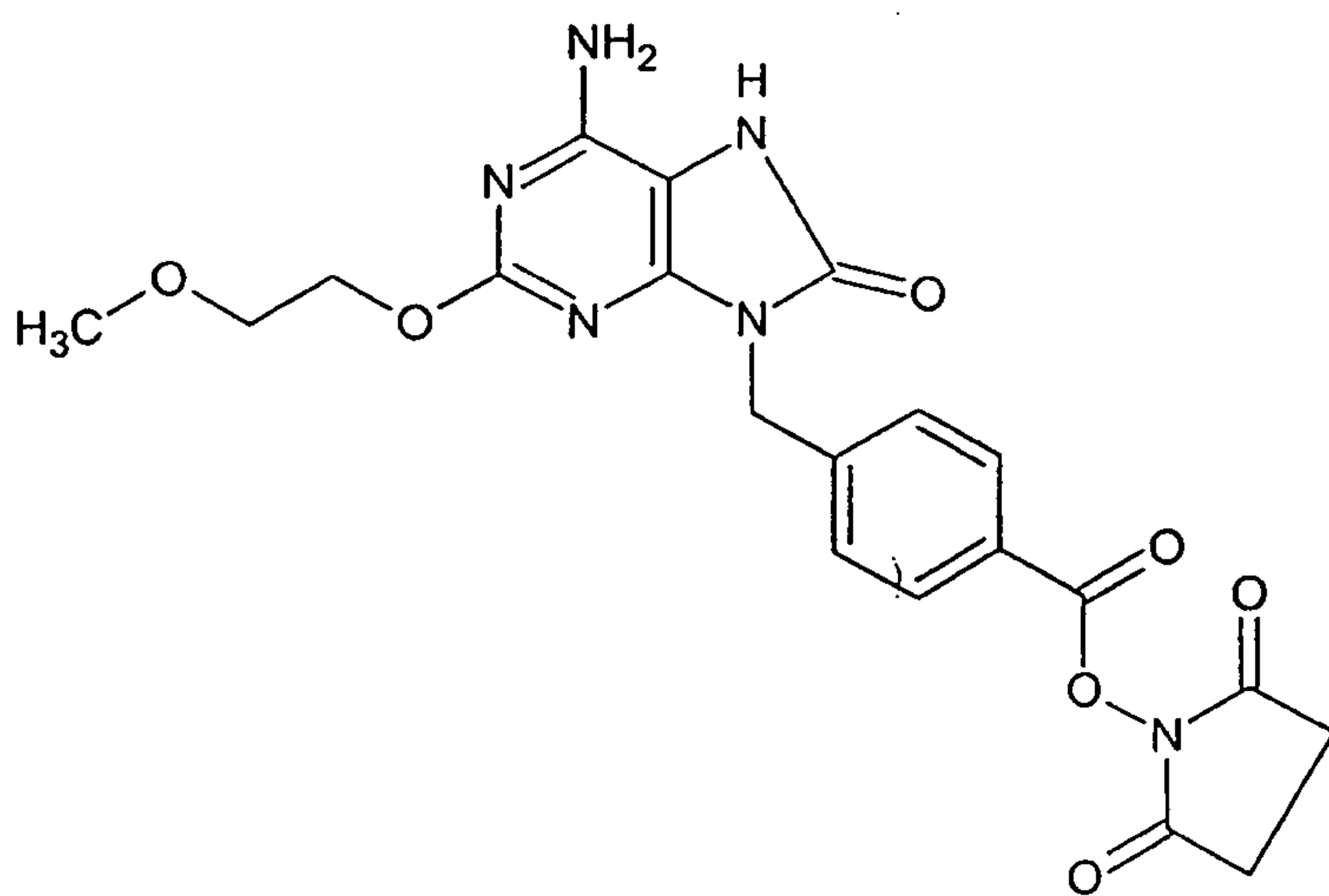
Bropirimine
