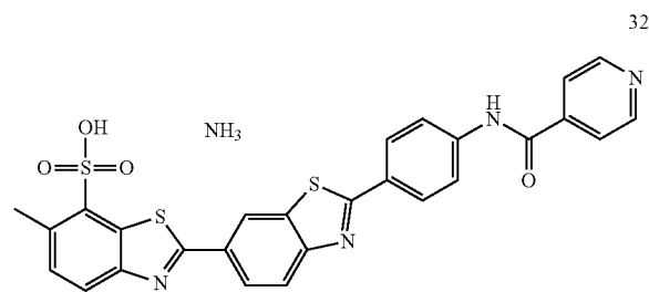
2'-(4-(isonicotinamido)phenyl)-6-methyl-[2,6'-bibenzo[d]thiazole]-7-sulfonic acid (32)
