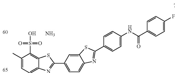
2'-(4-benzamidophenyl)-6-methyl-[2,6'-bibenzo[d]thiazole]-7-sulfonic acid (5)
