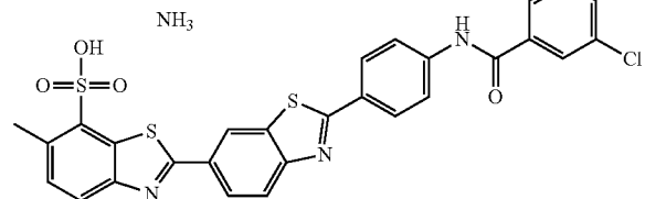
6-methyl-2'-(4-(2-(trifluoromethyl)benzamido)phenyl)-[2,6'-bibenzo[d]thiazole]-7-sulfonic acid (19)
