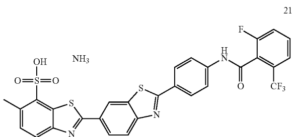
2'-(4-(2-fluoro-6-(trifluoromethyl)benzamido)phenyl)-6-methyl-[2,6'-bibenzo[d]thiazole]-7-sulfonic acid (21)
