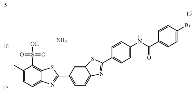
2'-(4-(4-bromobenzamido)phenyl)-6-methyl-[2,6'-bibenzo[d]thiazole]-7-sulfonic acid (15)
