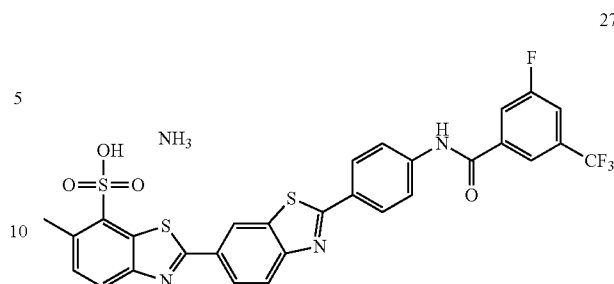
2'-(4-(3-fluoro-5-(trifluoromethyl)benzamido)phenyl)-6-methyl-[2,6'-bibenzo[d]thiazole]-7-sulfonic acid (27)
