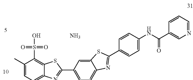
6-methyl-2'-(4-(nicotinamido)phenyl)-[2,6'-bibenzo[d]thiazole]-7-sulfonic acid (31)
