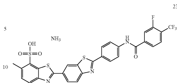
2'-(4-(3-fluoro-4-(trifluoromethyl)benzamido)phenyl)-6-methyl-[2,6'-bibenzo[d]thiazole]-7-sulfonic acid (23)
