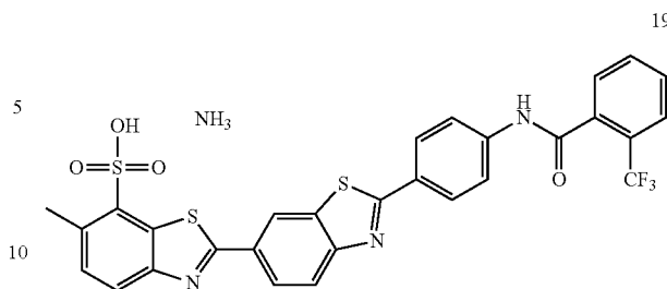
6-methyl-2'-(4-(2-(trifluoromethyl)benzamido)phenyl)-[2,6'-bibenzo[d]thiazole]-7-sulfonic acid (19)
