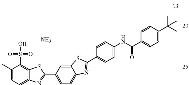
2'-(4-(4-(tert-butyl)benzamido)phenyl)-6-methyl-[2,6'-bibenzo[d]thiazole]-7-sulfonic acid (13)
