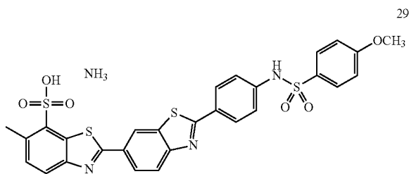
2'-(4-(4-methoxyphenyl)sulfonamido)phenyl)-6-methyl-[2,6'-bibenzo[d]thiazole]-7-sulfonic acid (29)
