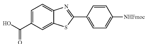
2'-(4-((9H-fluorene-9-yl)methoxy)carbonylamino)phenyl)benzo[d]thiazole-6-carboxylic acid (39)
