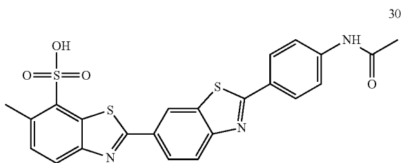
2'-(4-acetamidophenyl)-6-methyl-[2,6'-bibenzo[d]thiazole]-7-sulfonic acid (30)
