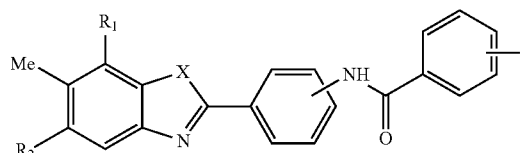
Formula II
