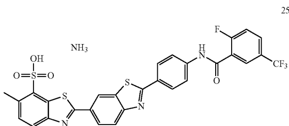
2'-(4-(2-fluoro-5-(trifluoromethyl)benzamido)phenyl)-6-methyl-[2,6'-bibenzo[d]thiazole]-7-sulfonic acid (25)
