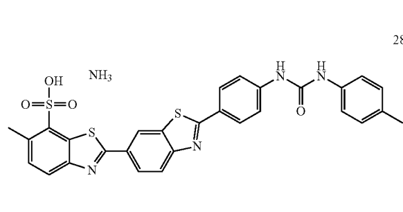
6-methyl-2'-(4-(3-(p-tolyl)ureido)phenyl)-[2,6'-bibenzo[d]thiazole]-7-sulfonic acid (28)
