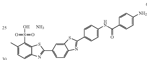
2'-(4-(4-aminobenzamido)phenyl)-6-methyl-[2,6'-bibenzo[d]thiazole]-7-sulfonic acid (6)
