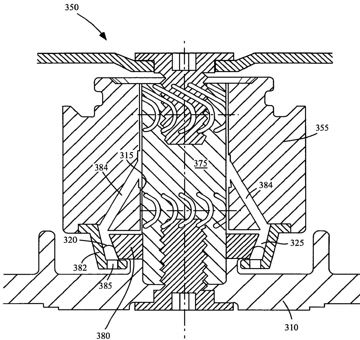
FIG. 3 (Prior Art)
