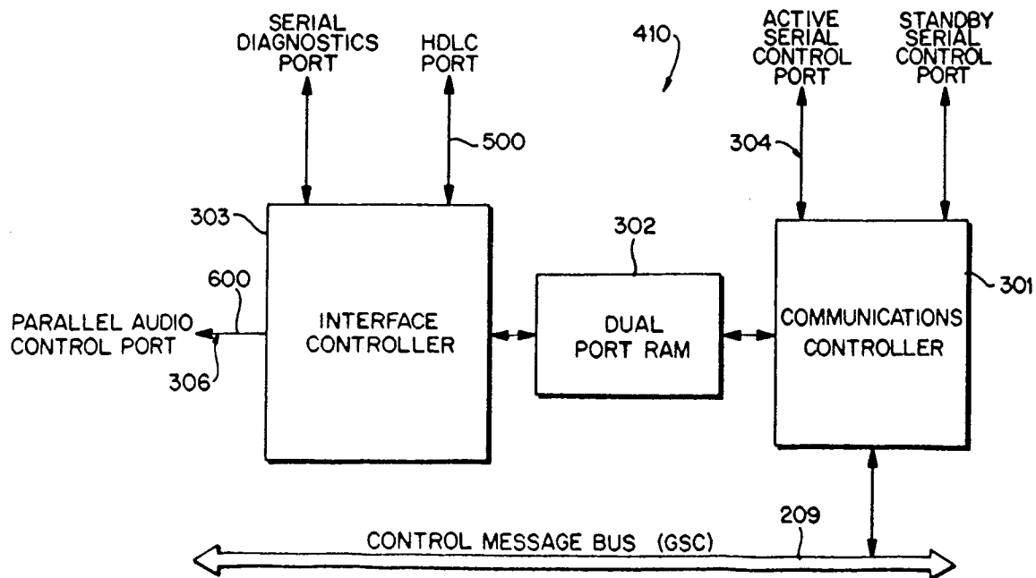
FIG. 4 SWITCH CONTROLLER CARD ARCHITECTURE
