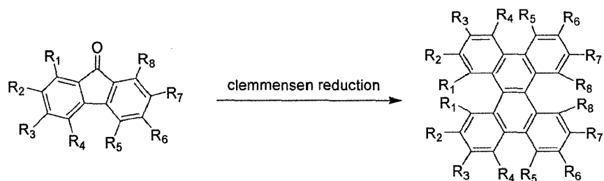
Reaction Scheme 1
