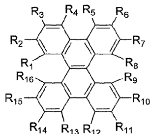
Chemical Formula 1
