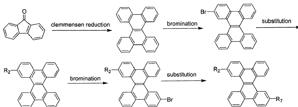
Reaction Scheme 3
