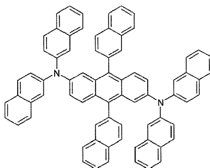
Compound E
