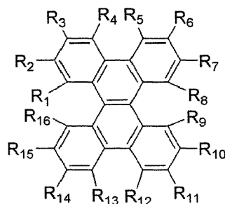
Chemical Formula 1
