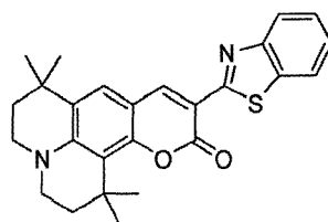
Chemical Formula 4
