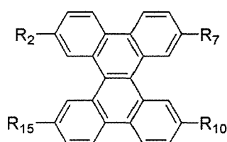
Chemical Formula 2
