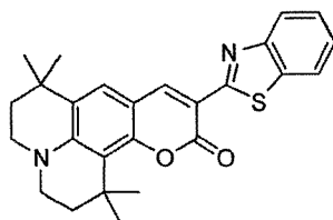
Chemical Formula 4
