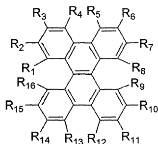
Chemical Formula 1
