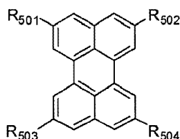
Chemical Formula 3
