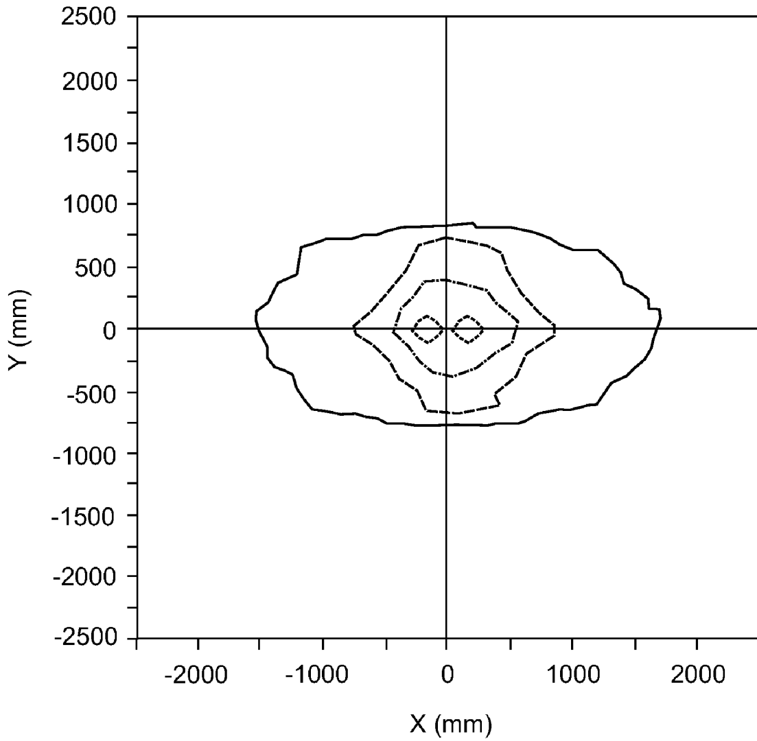
Illuminance Chart
