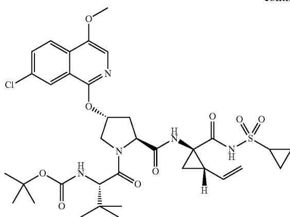
BMS-650032 (Asunaprevir)
