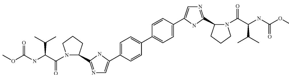
Daclatasvir dihydrochloride
