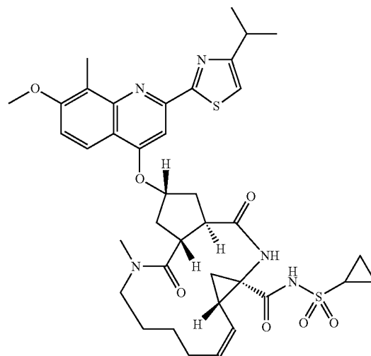
TMC-435 (TMC-435350)
