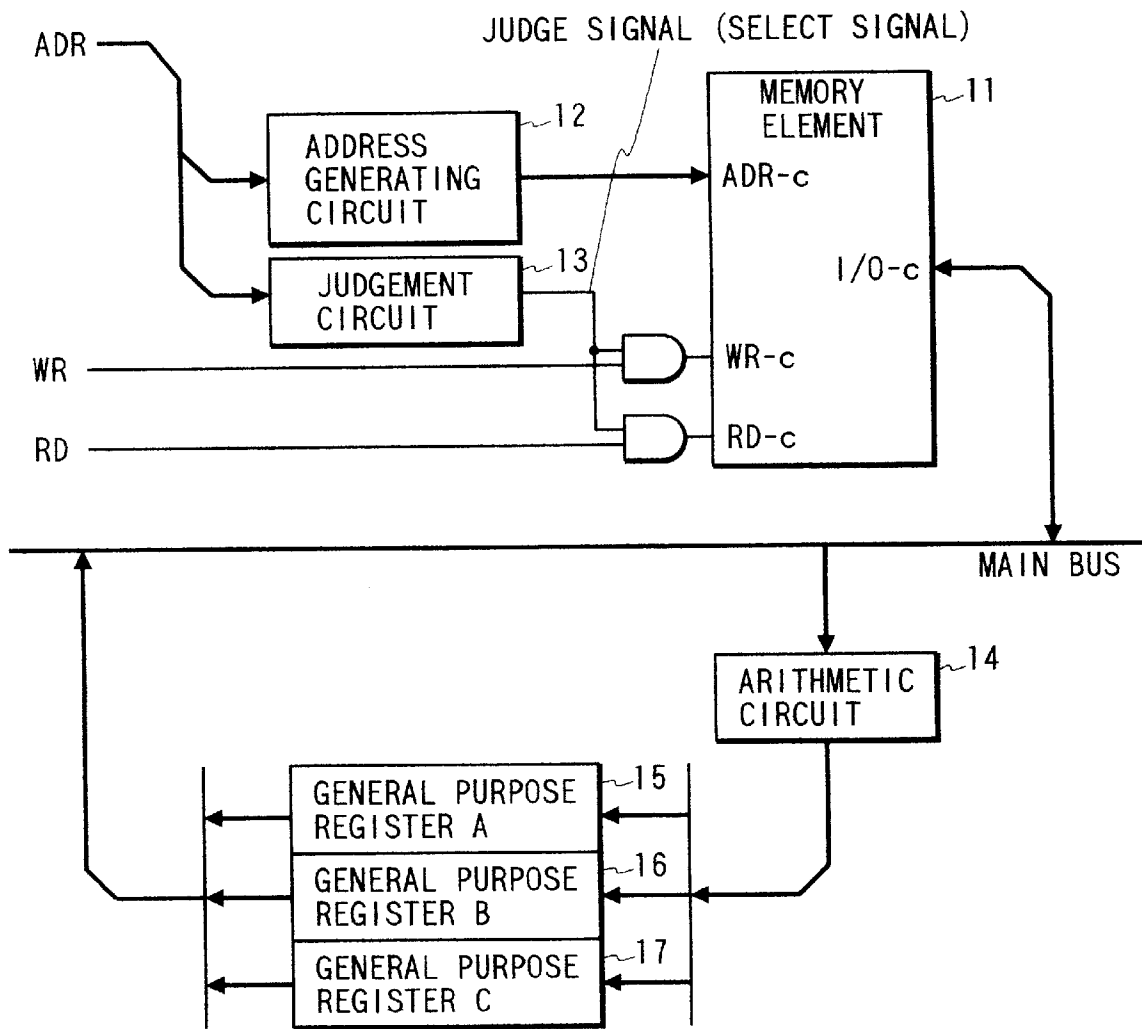
FIG. 1 PRIOR ART
