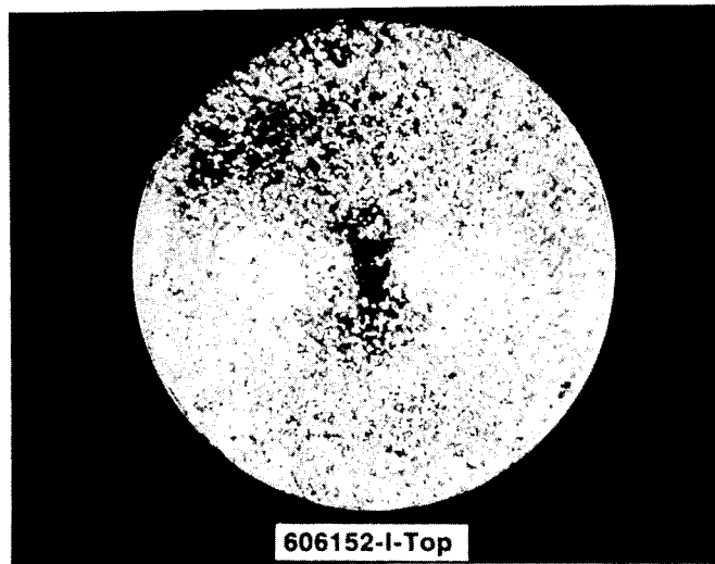
Macroetched Grain Appearance of a 6" Round Ingot Cast With Multiple Slanted Feed Openings Around the Prepherel of the Casting Basin
