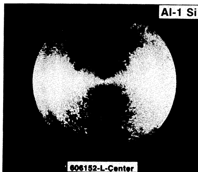
A Typical Macroetched Grain Structures of 6" Round Ingots Cast by Incorporating Mechanical Stirring for a) Al-2 Cu, and b) Al-1 Si Alloys FIG. 6
