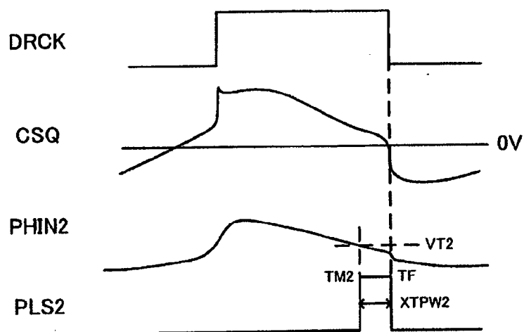
FIG. 14B MEDIUM LOAD
