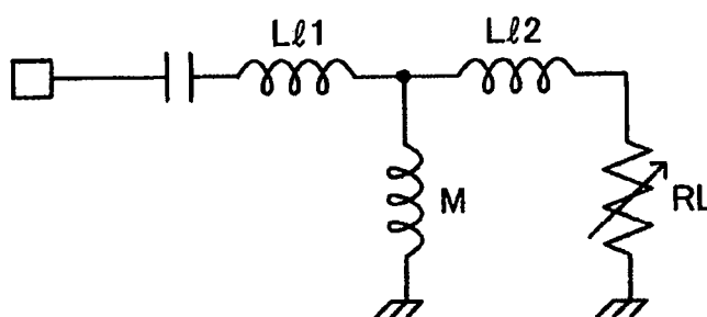
FIG. 10B LOAD-CONNECTED
