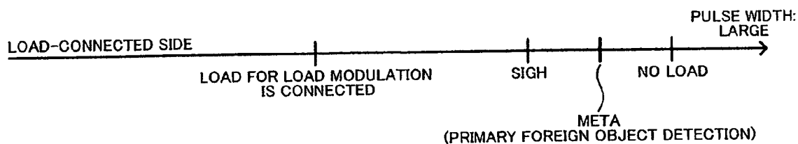
FIG. 18B SECOND LOAD STATE DETECTION CIRCUIT (PWQ2)
