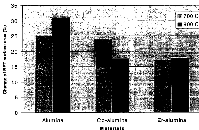
Comparison of Hydrothermal Stability of Coprecipitated Alumina
