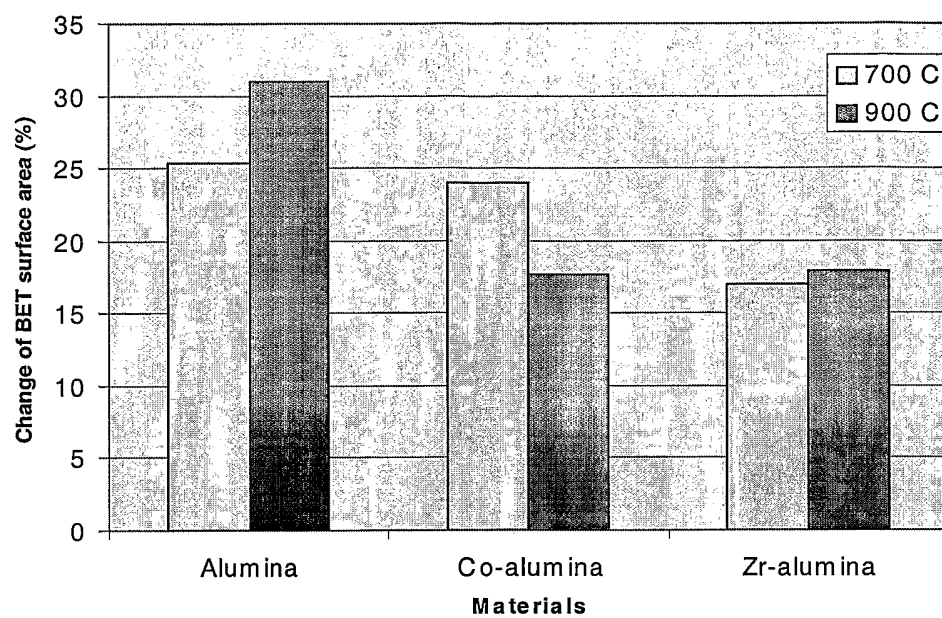
Comparison of Hydrothermal Stability of Coprecipitated Alumina
