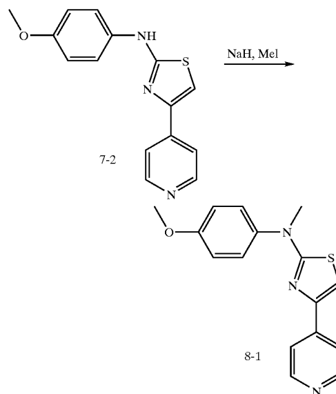
SCHEME 8
