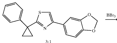
SCHEME 3
