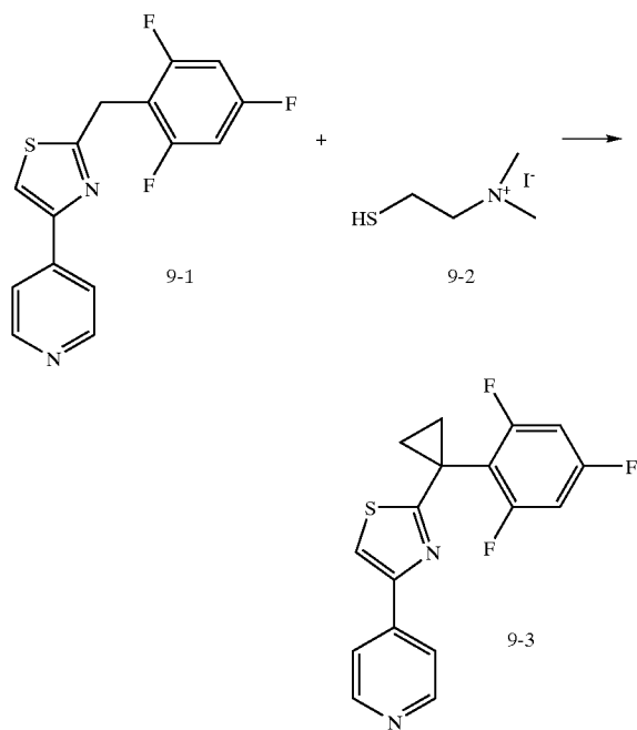
SCHEME 9
