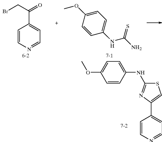
SCHEME 7
