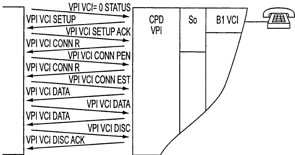
FIGURE 7: CONNECTION PROCESS WHEN THE SU REQUESTS A CONNECTION
