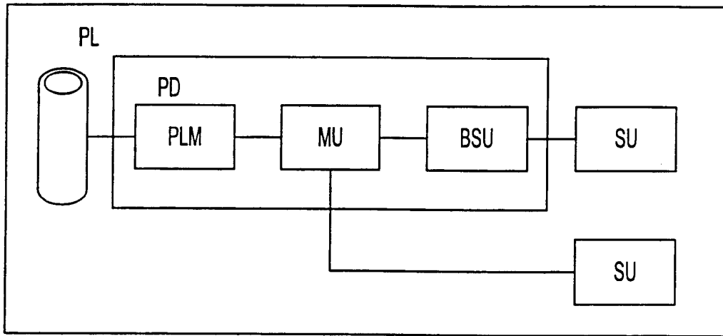
FIGURE 3: STRUCTURE OF A POWERLINE DEVICE (PLM-POWERLINE MODEM, MU-MANAGEMENT UNIT, BSU-BASIC SERVICE UNIT, SU-SERVICE UNIT)
