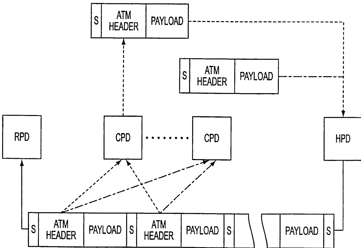
FIGURE 4: TRANSMIT AND RECEIVE IN THE PL-NETWORK (S-SYNCHRONIZATION)
