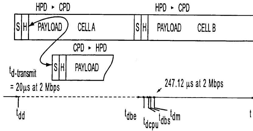
FIGURE 11: TRANSMISSION SYNCHRONIZATION AND DELAY TIMES
