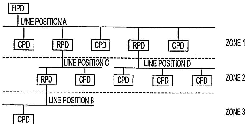
FIGURE 2: HIERARCHICAL BUS STRUCTURE OF THE PL-SYSTEM (RPD REPEATER POWERLINE DEVICE)
