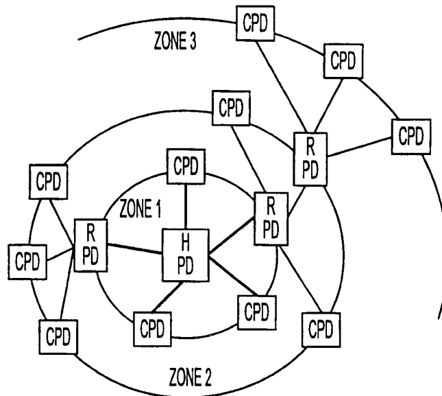
FIGURE 12: ZONE STRUCTURE OF THE NETWORK (RPD-REPEATER POWERLINE DEVICE)
