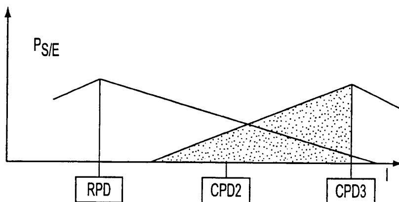
FIGURE 8: PROBLEM OF MULTIPLE UTILIZATION OF LINE POSITIONS
