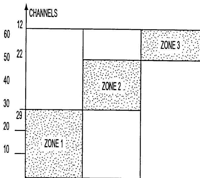
FIGURE 9: BANDWIDTHS IN THE VARIOUS ZONES DEPENDENT ON THE ACTIVE SU CHANNELS
