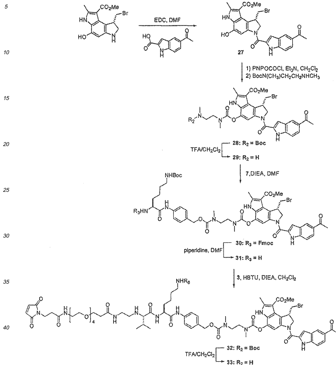
Scheme 6
