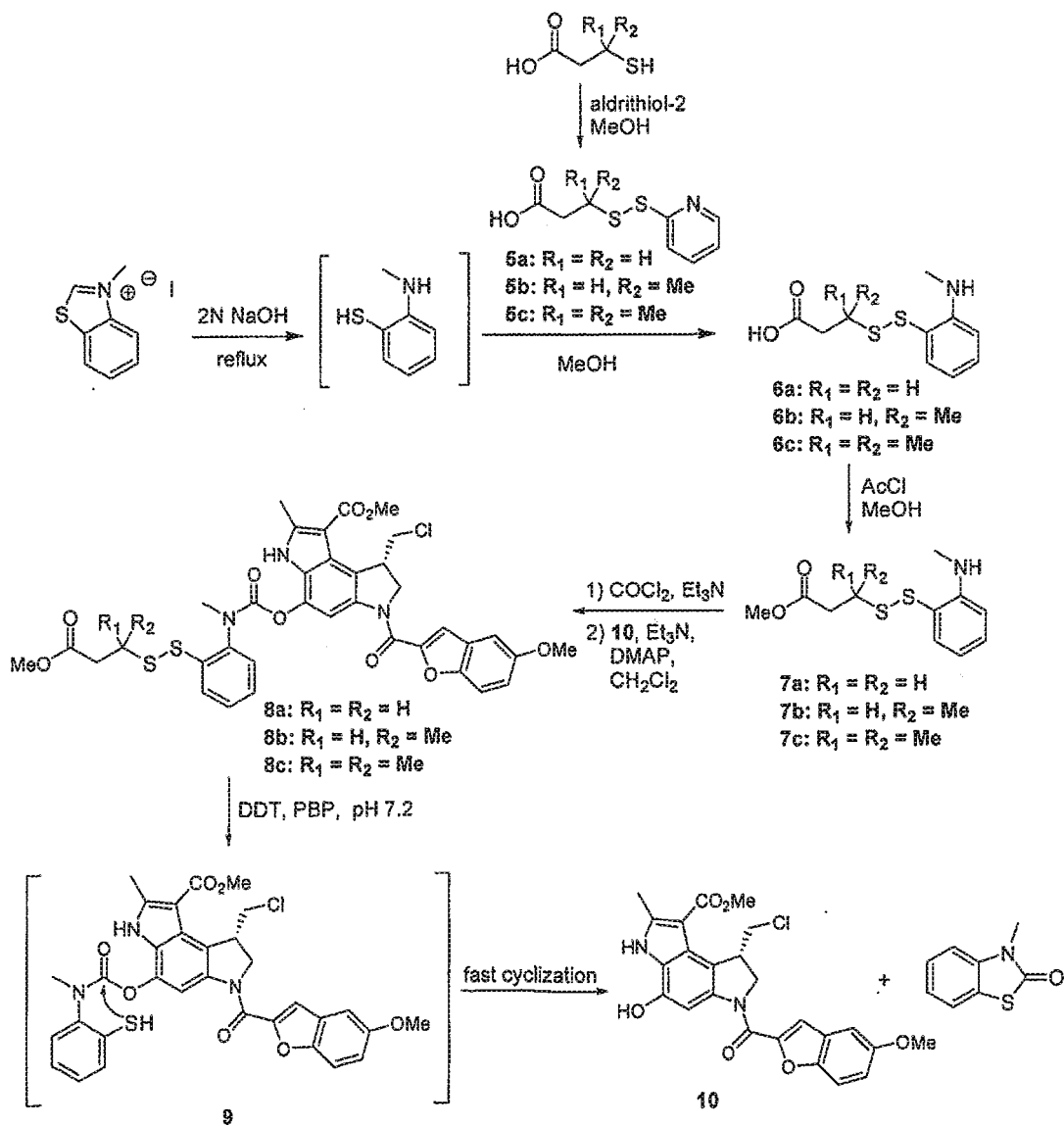
Scheme 2
