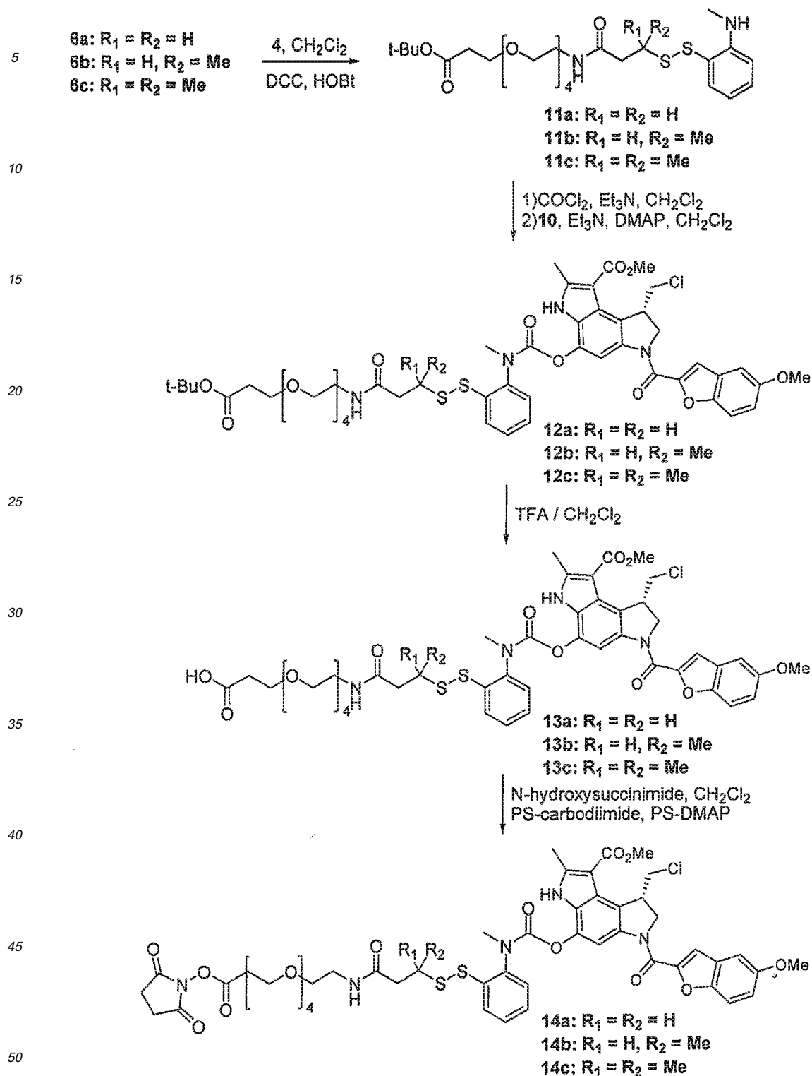
Scheme 3
