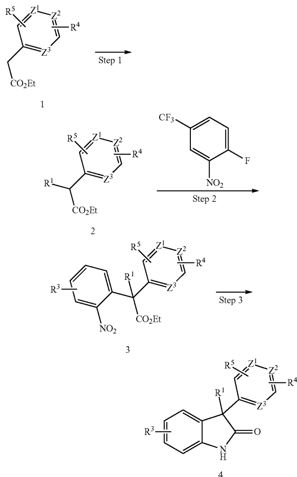
Scheme 2: General method for the preparation of 3-heteroaryl-3-alkyl-indolin-2-ones.
