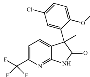
Example 37: 3-(5-chloro-2-methoxyphenyl)-3-methyl-6-(trifluoromethyl)-1H-pyrrolo[3,2-c]pyridin-2(3H)-one
