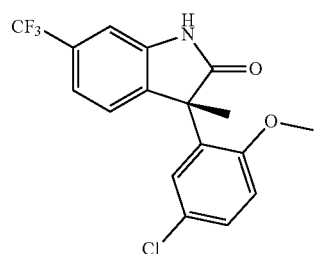
(3S)-3-(5-chloro-2-methoxyphenyl)-3-methyl-6-(trifluoromethyl)indolin-2-one
