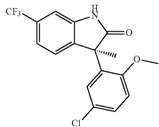
(3R)-3-(5-chloro-2-methoxyphenyl)-3-methyl-6-(trifluoromethyl)indolin-2-one
