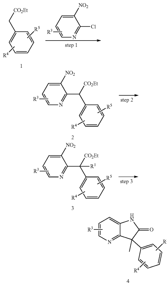
Scheme 3: General method for the preparation of
