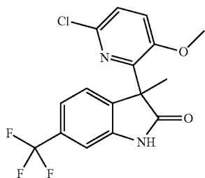
Example 27: 6-chloro-3-(5-chloro-2-methoxyphenyl)-3-methyl-1H-pyrrolo[3,2-c]pyridin-2(3H)-one
