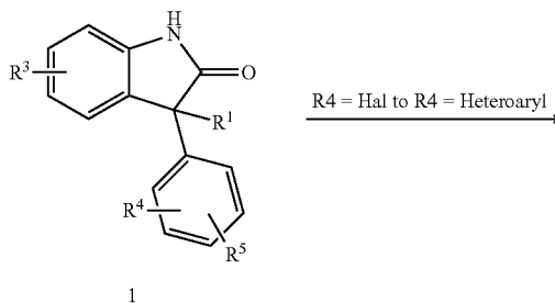
Scheme 8: General method for functionalization of 3-alkyl-indolin-2-ones.
