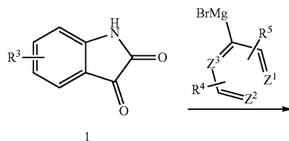
Scheme 7: General method for the preparation of 3-heteroaryl-3-alkyl-indolin-2-ones.
