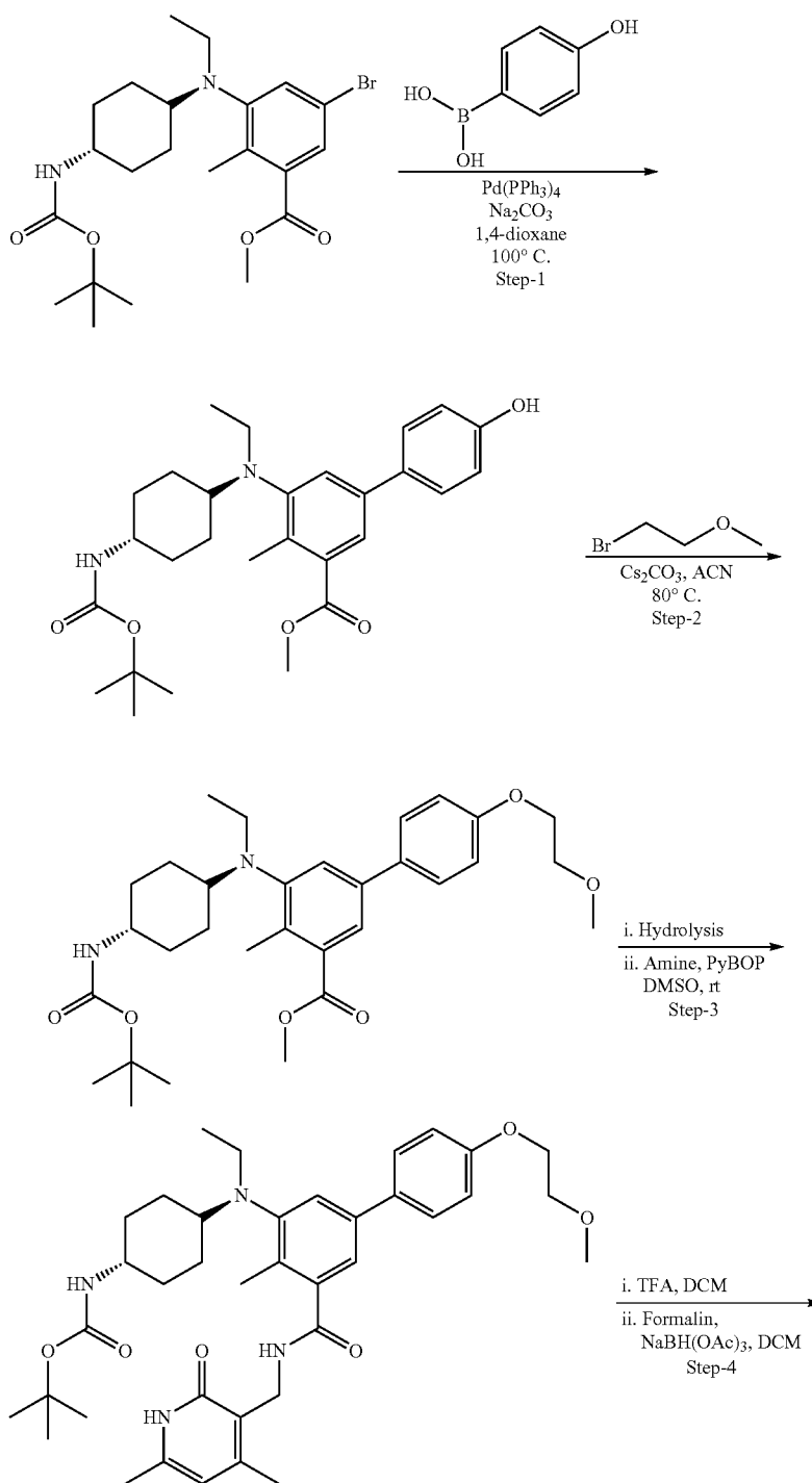
Compound 1:
