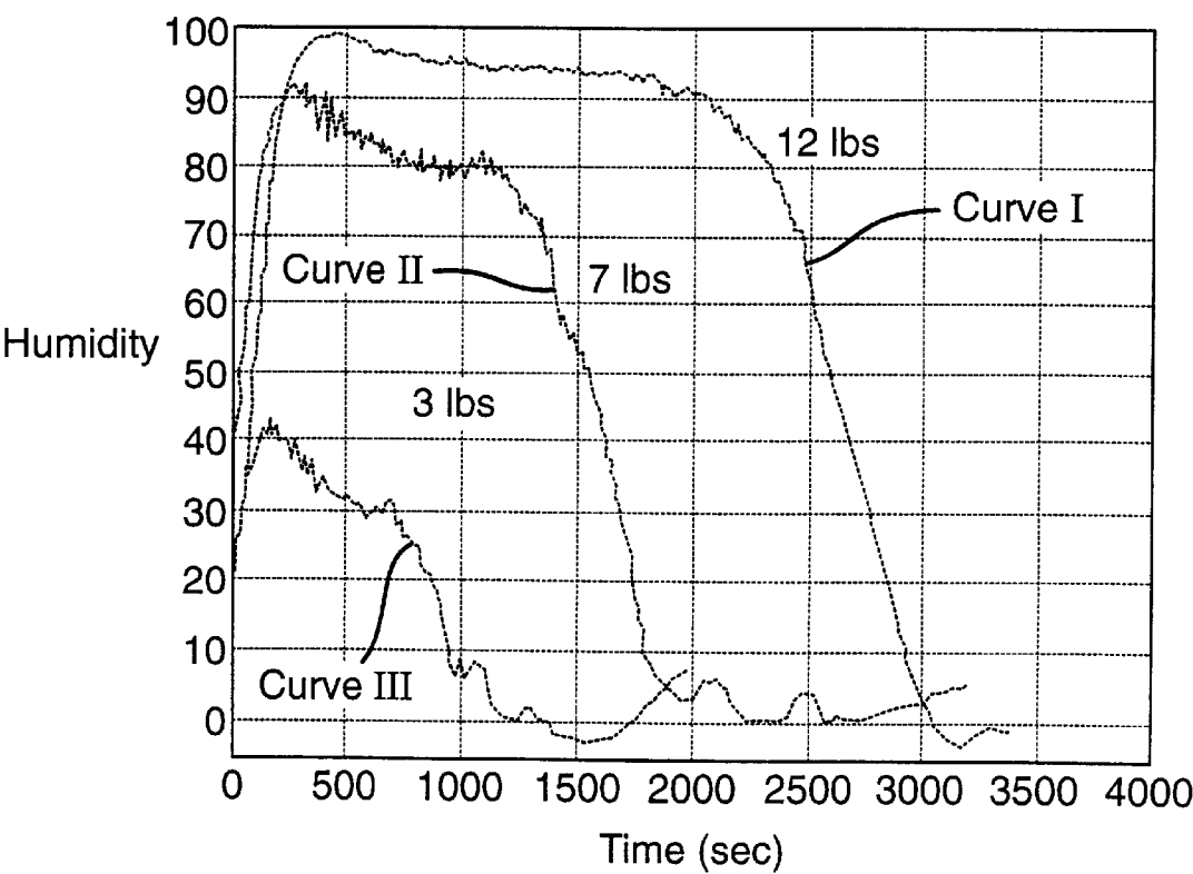
Humidity Vs. Drying Time For Different Loads
