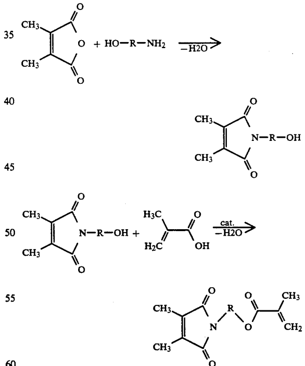
FIG. 4: DMMI Monomer Synthesis
