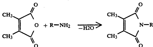
FIG. 2: Synthesis of DMMIs
