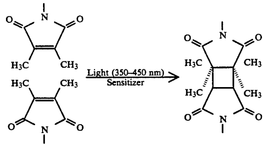
FIG. 3: Photo Induced Cyclo-addition Reaction of DMMI's
