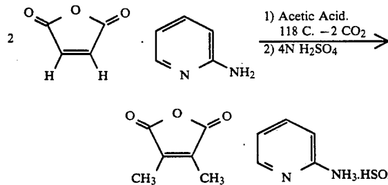
FIG. 1: Synthesis of DMMA
