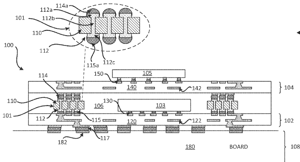
CROSS SECTIONAL PROFILE VIEW
