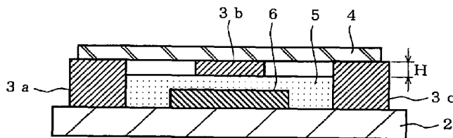
(x - x cross section)
