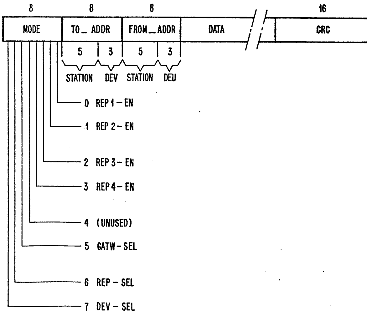
FIG. 7 PACKET FORMAT
