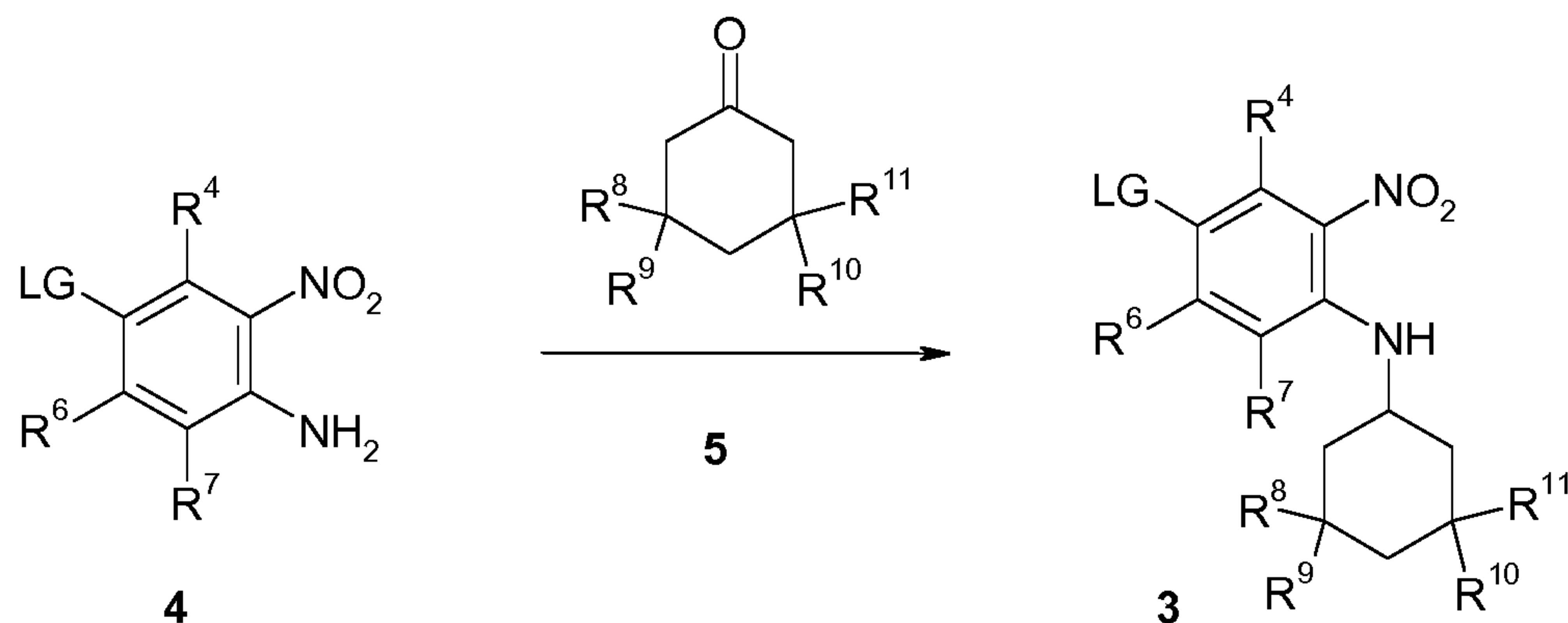
Scheme 2:
