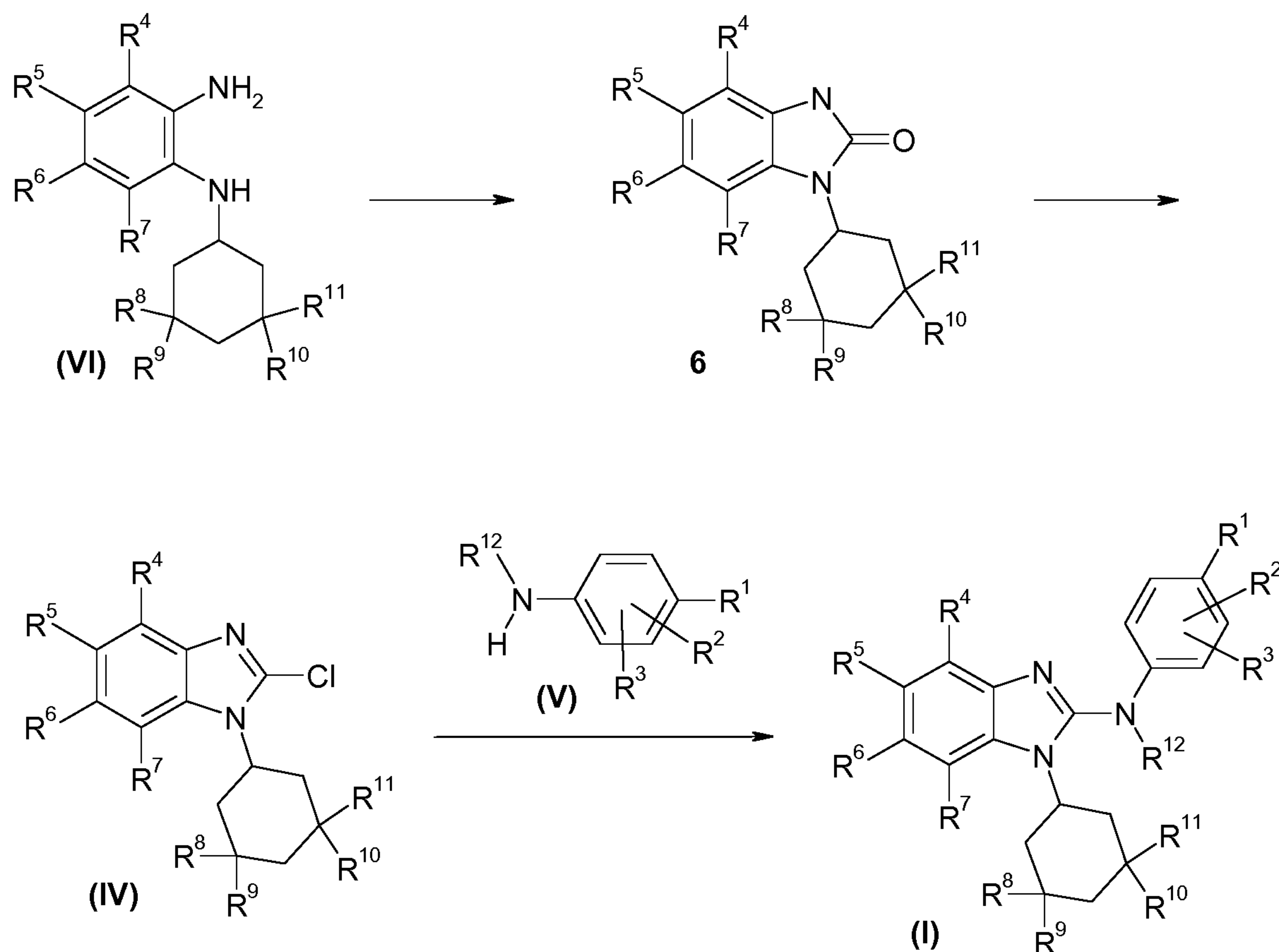
Scheme 3:
