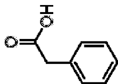
Phenyl-Acetic Acid
