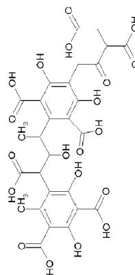
Humic Acid
