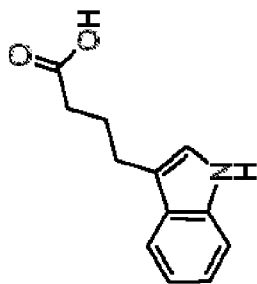
Indole-Butyric Acid
