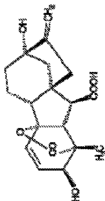
Gibberellic Acid
