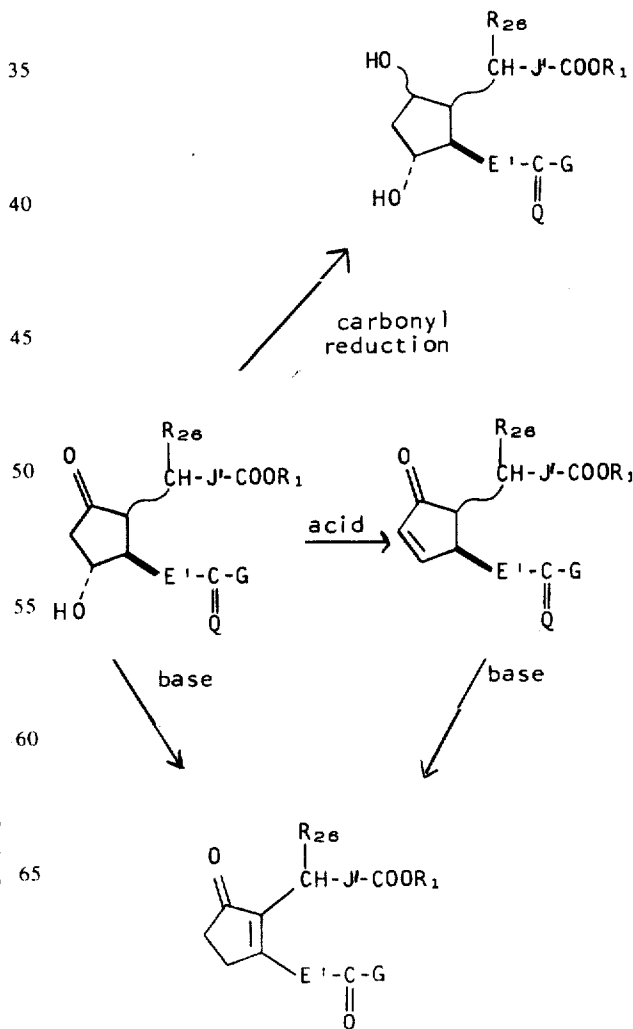
CHART A
