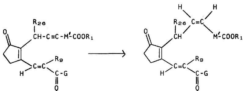
CHART D
