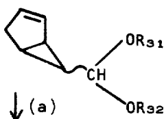
CHART M
