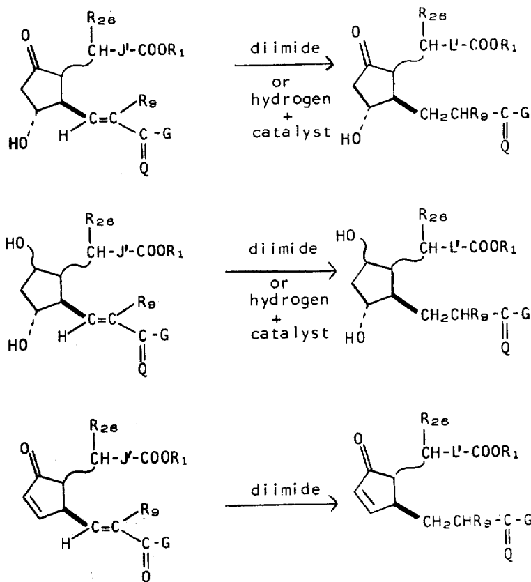
CHART B
