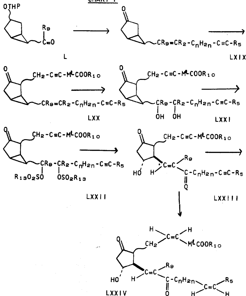
CHART F
