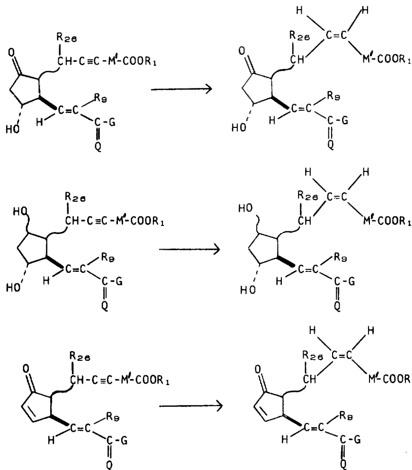
CHART C
