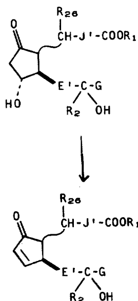
CHART K
