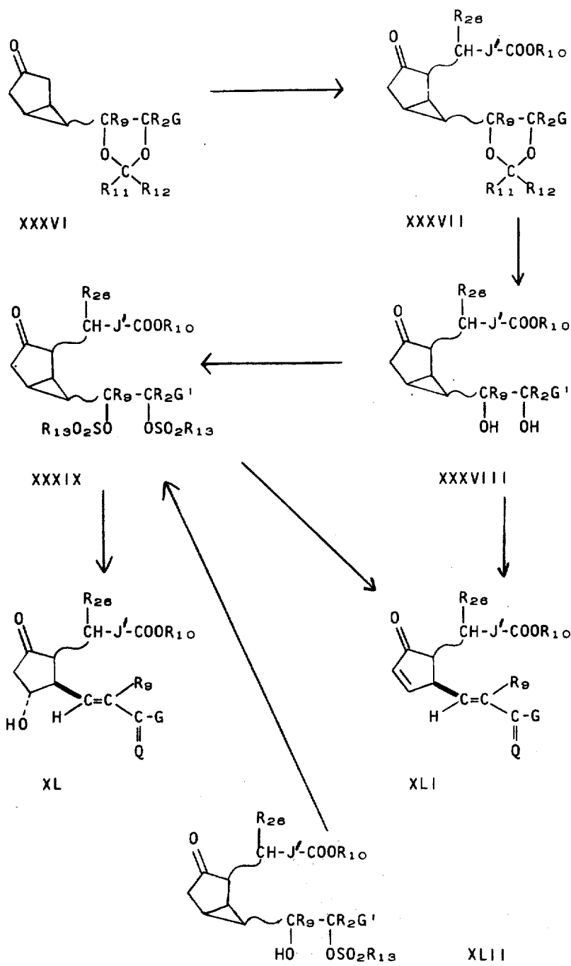
CHART D
