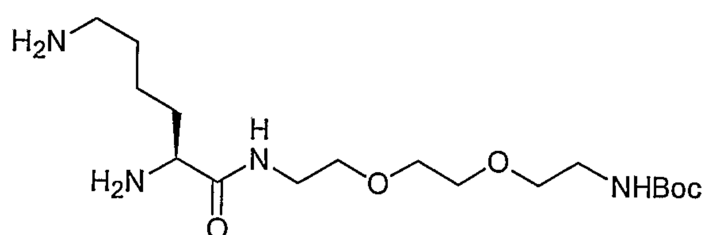
Formula VIII
