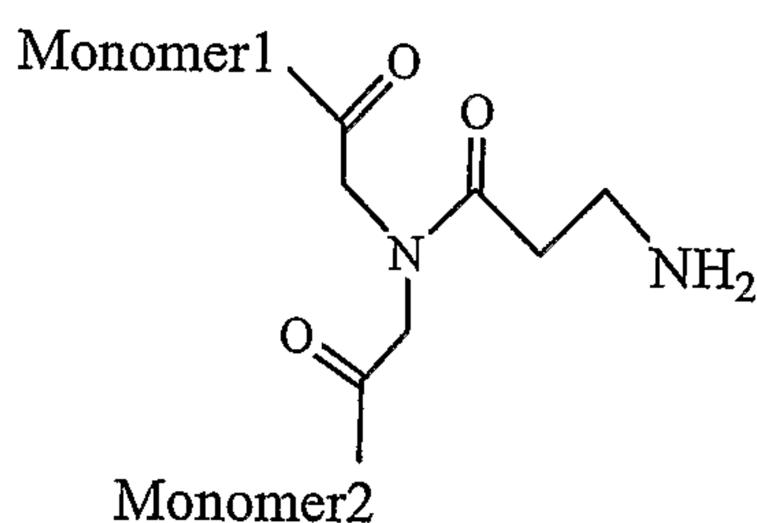
Formula IV
