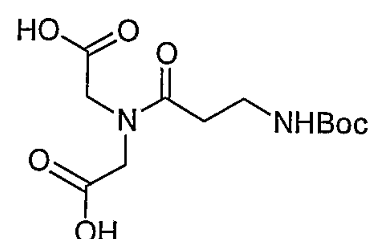
Formula IX
