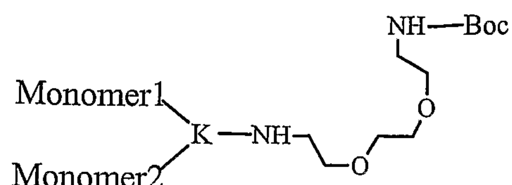
Formula VII
