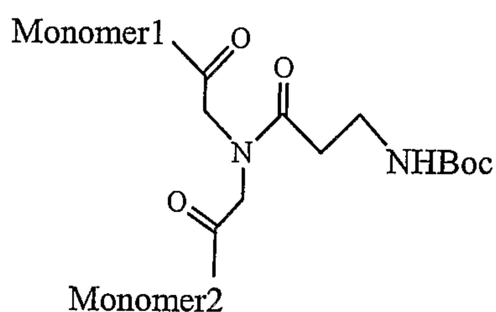
Formula III
