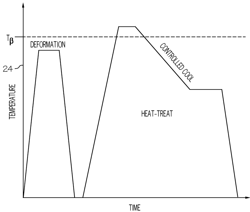
FIG. 2 (PRIOR ART)
