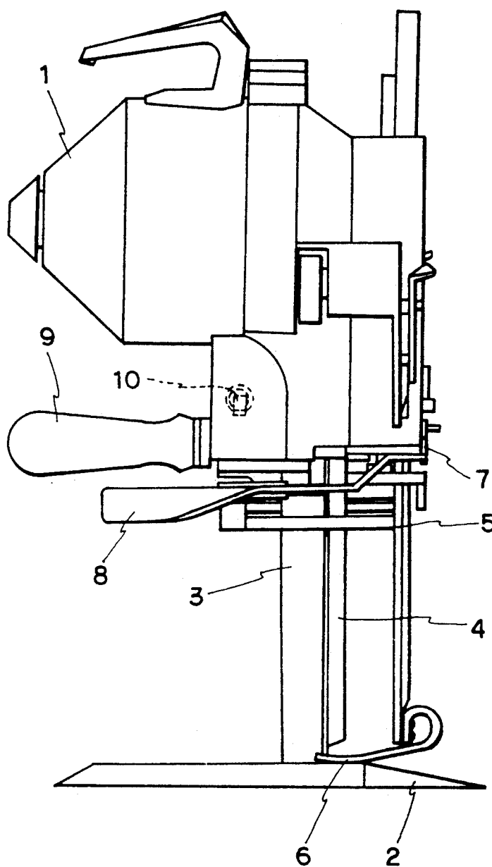
PRIOR ART Fig. 5
