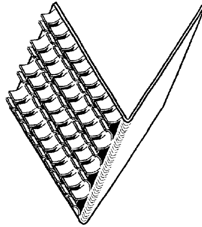
Fig. 3 - Angle view of baffle
