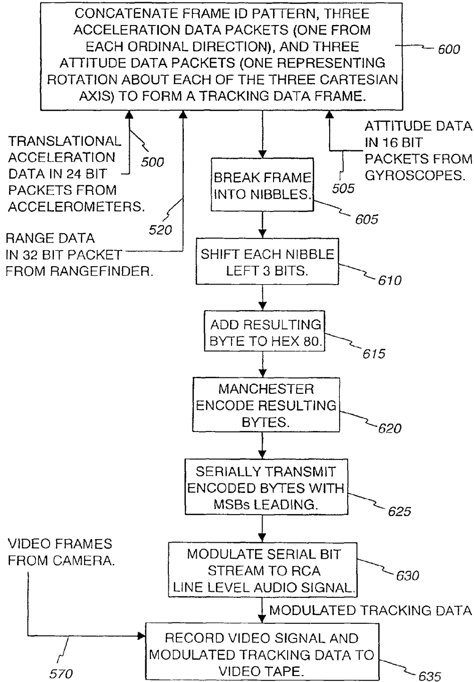
TRACKING DATA ACQUISITION UNIT DATA FLOW DIAGRAM
