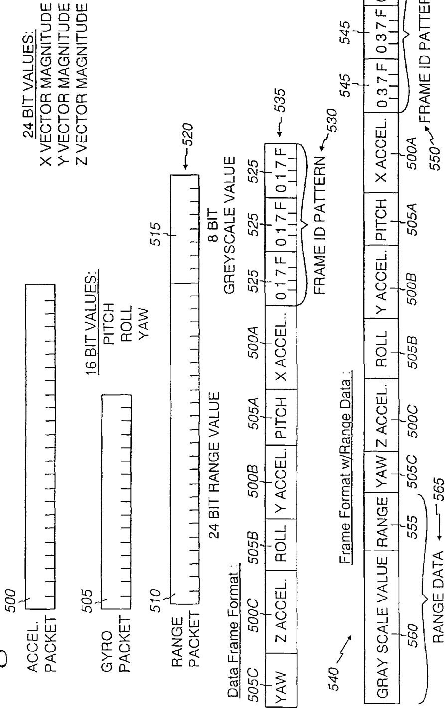
Fig. 4 TRACKING DATA ACQUISITION UNIT - DATA FORMAT DIAGRAM
