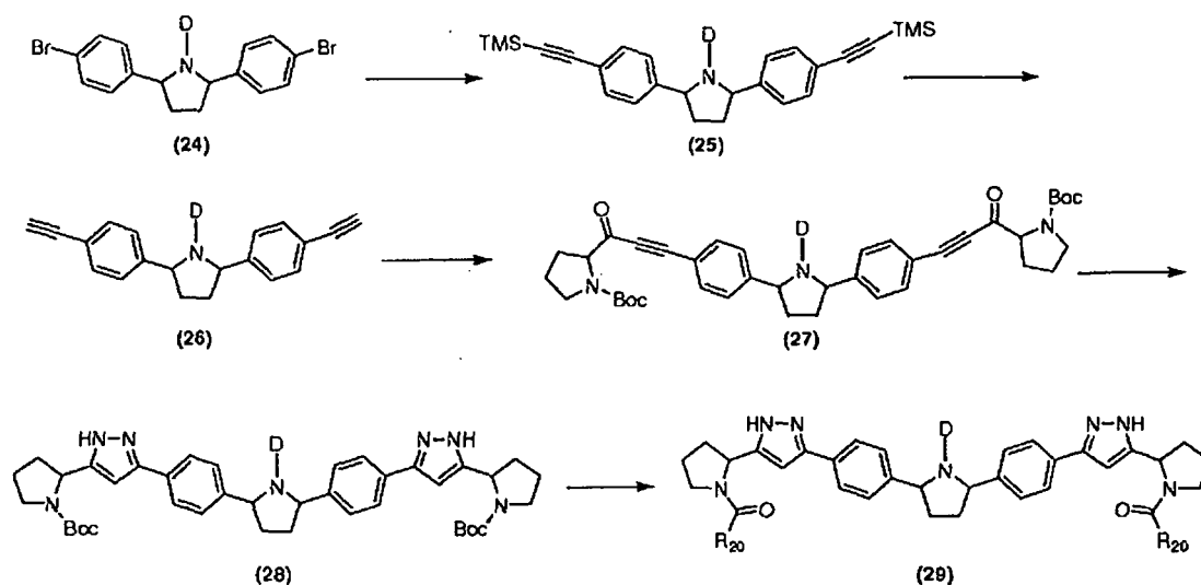
Scheme XV
