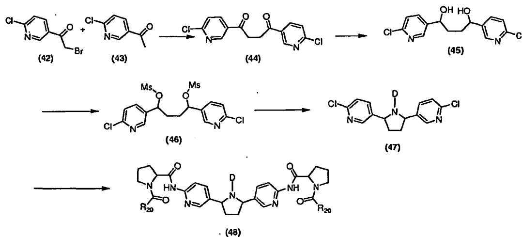
Scheme XIX
