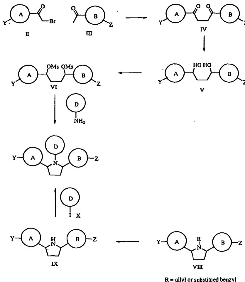
Scheme III
