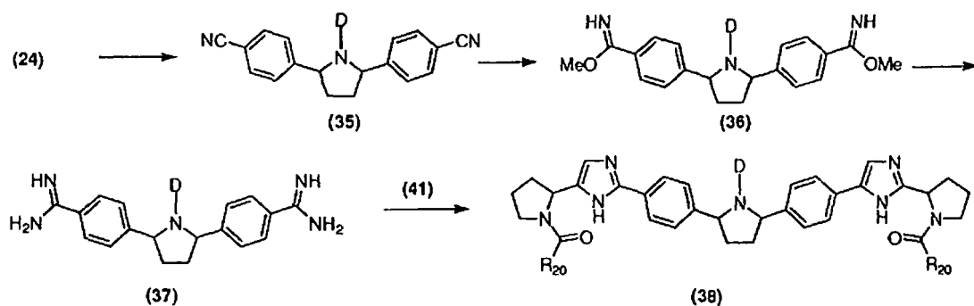
Scheme XVII
