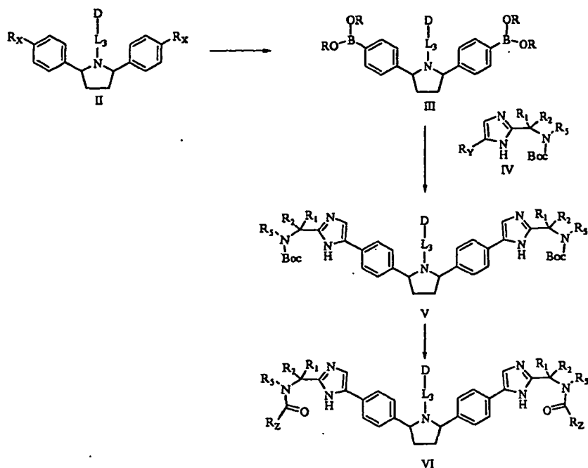
Scheme VII
