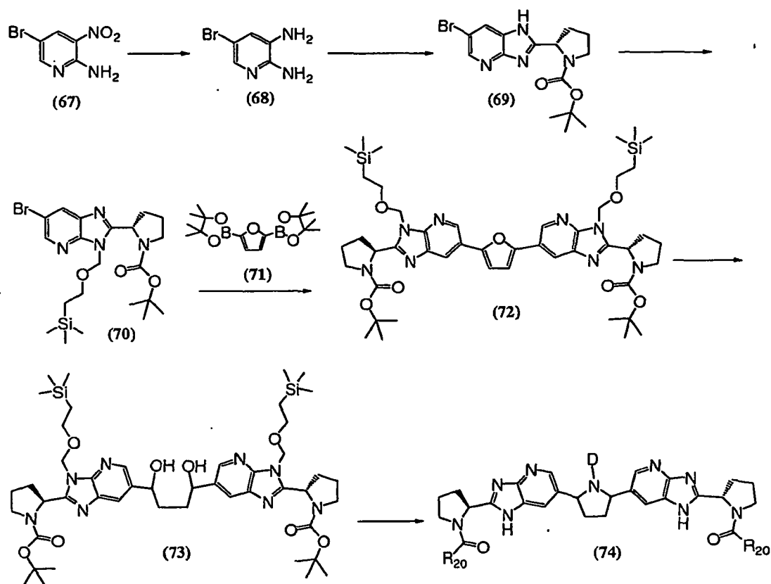
Scheme XXIII
