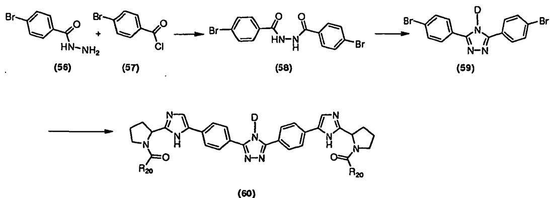
Scheme XXI
