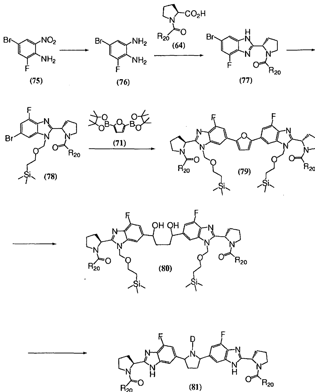
Scheme XXIV
