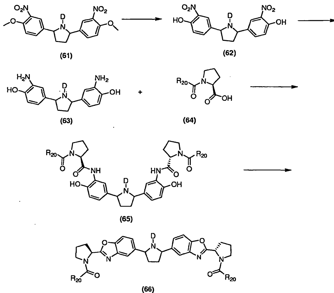
Scheme XXII
