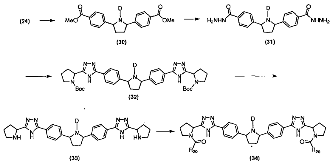
Scheme XVI
