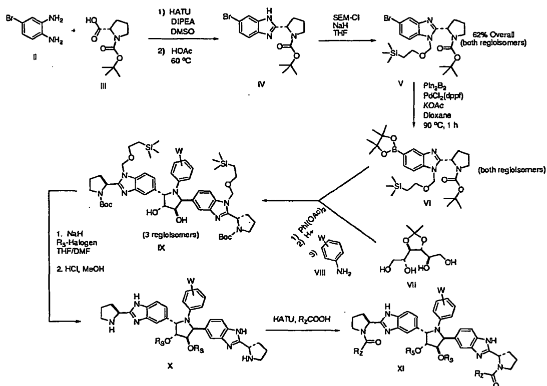
Scheme IX
