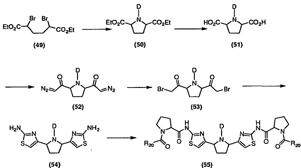
Scheme XX
