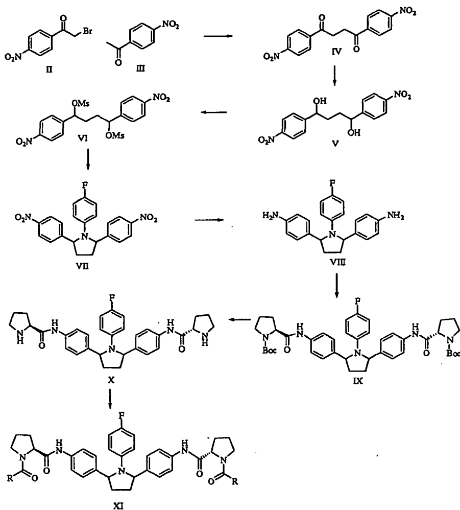
Scheme II
