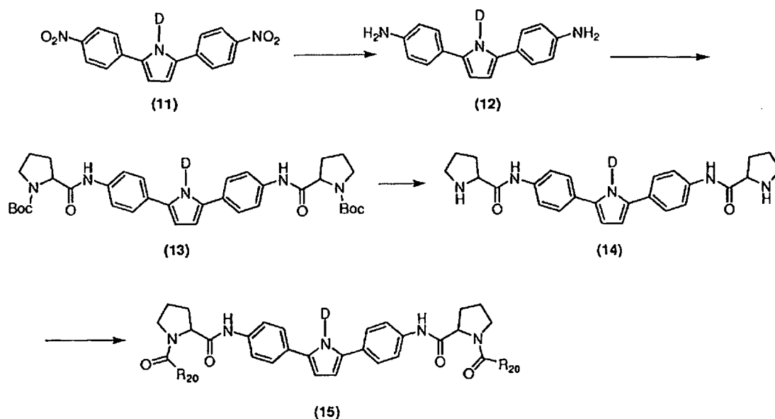
Scheme XII
