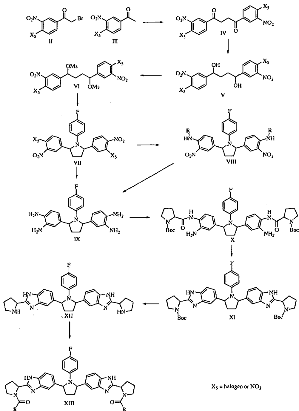
Scheme IV
