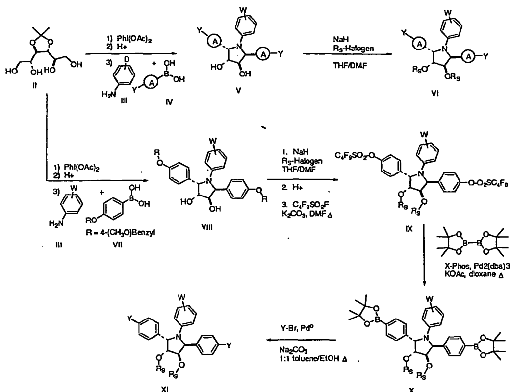
Scheme VIII
