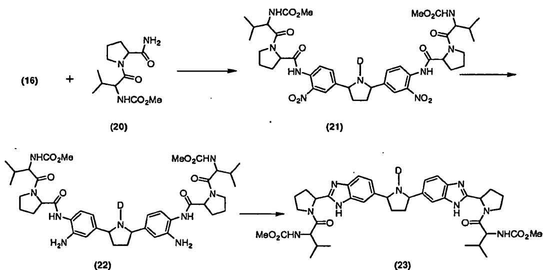
Scheme XIV
