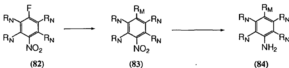
Scheme XXV
