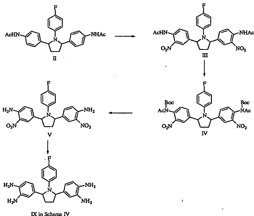
Scheme V
