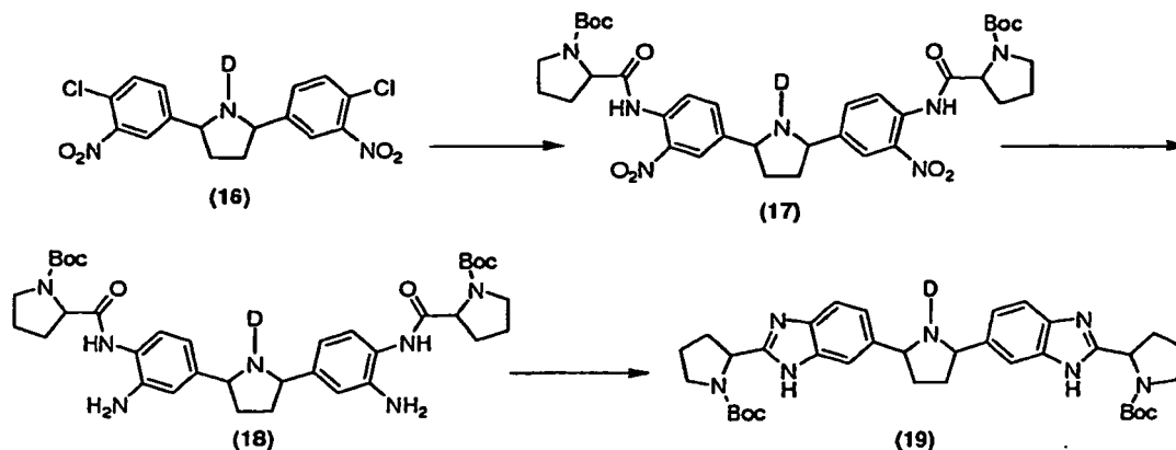
Scheme XIII
