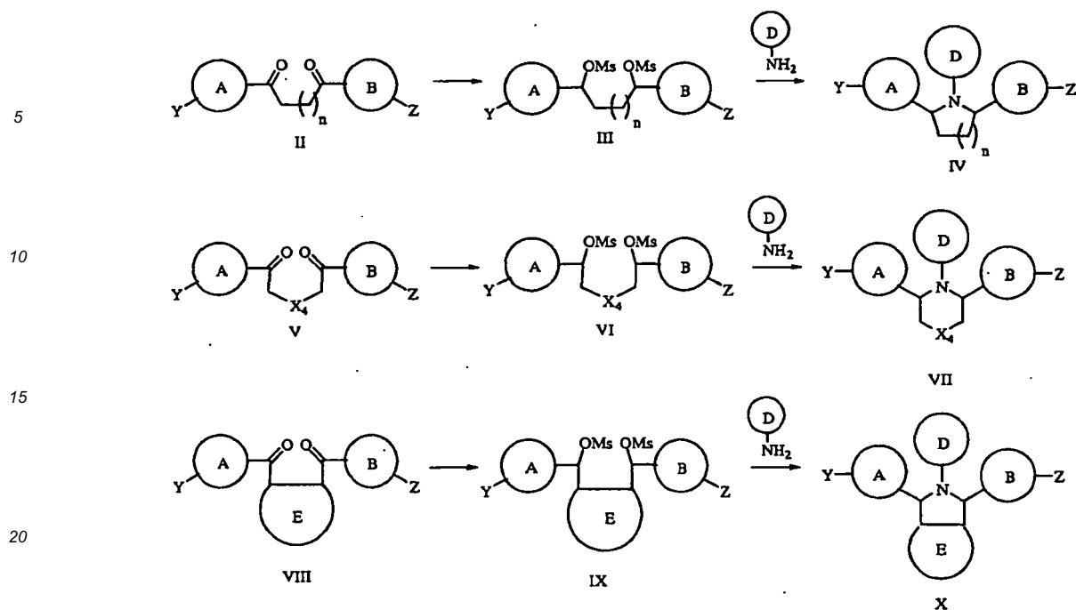
Scheme I
