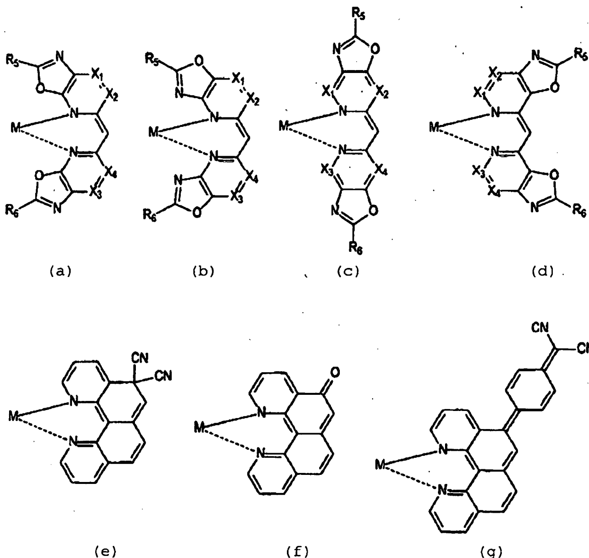
Formel 9
