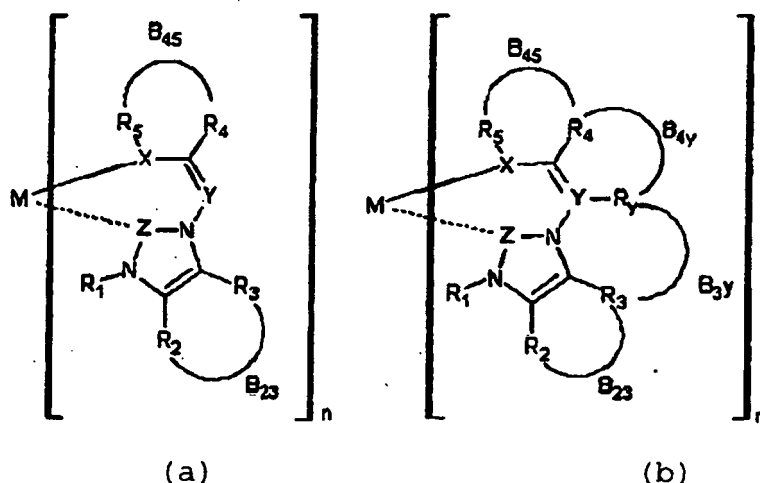
Formel 13
