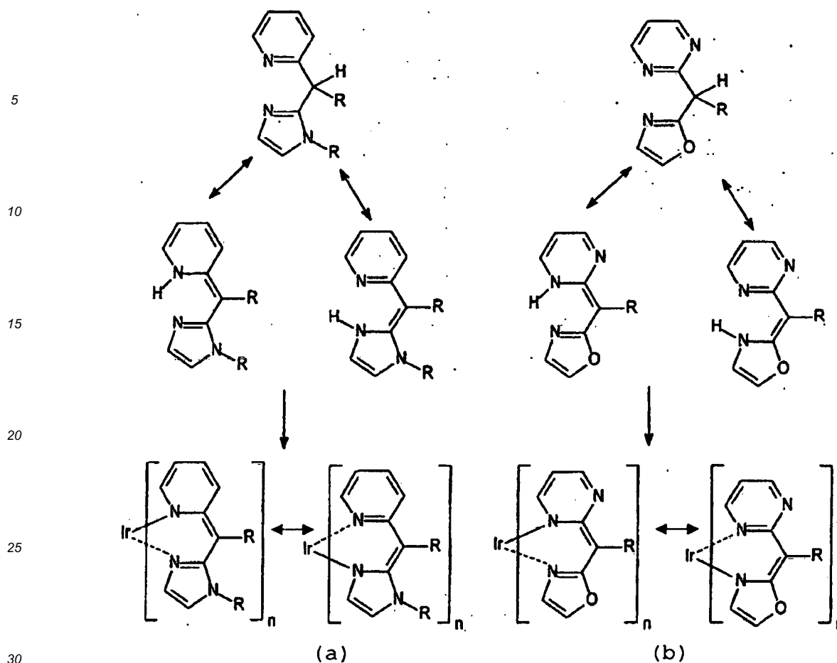
Formel 19
