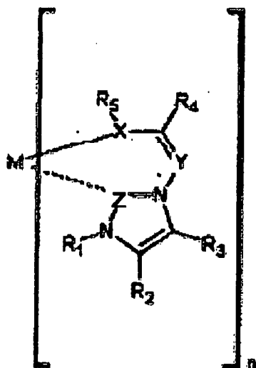
Formel 12
