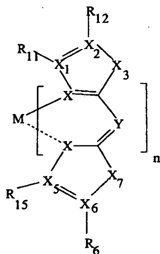
Formel 10
