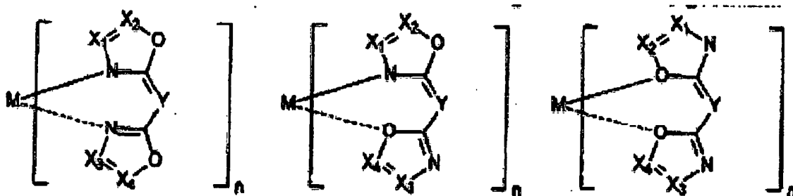
Formel 11
