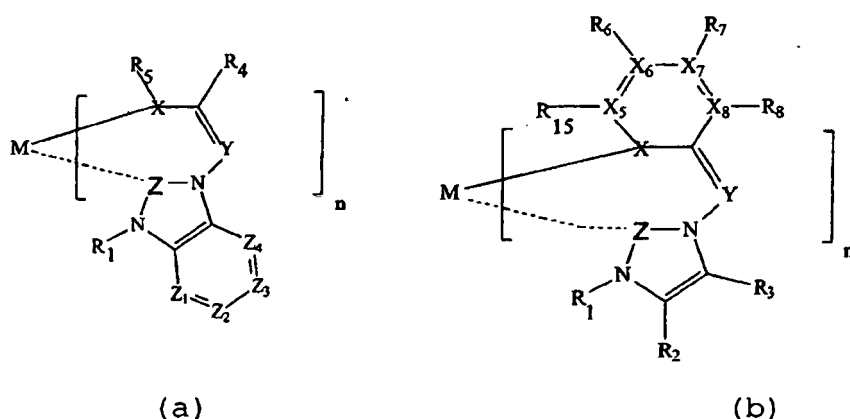
Formel 14
