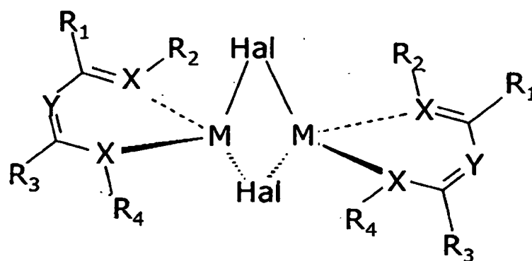
Formel 23
