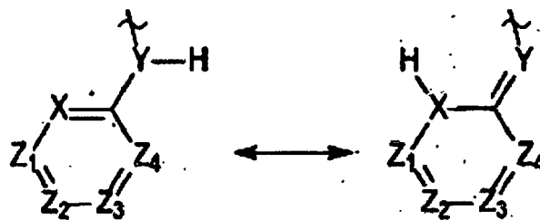
Formel 21
