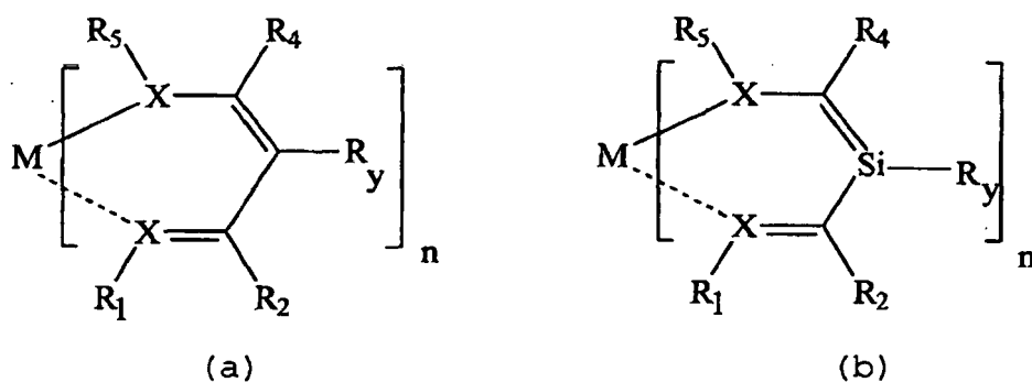
Formel 5
