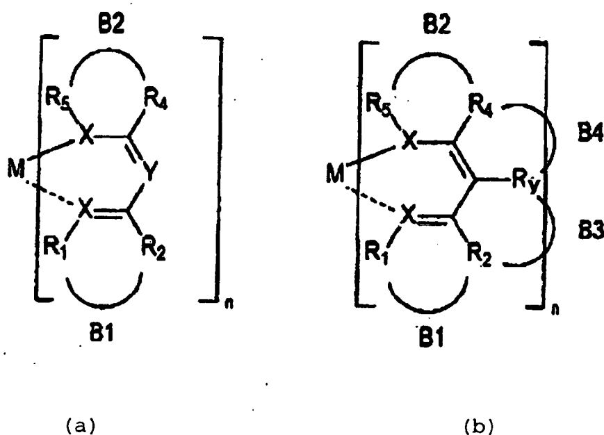
Formel 6
