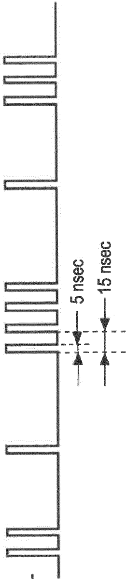
FIG. 5A WRITE STRATEGY SIGNAL (SHORT PULSE TRAIN)
