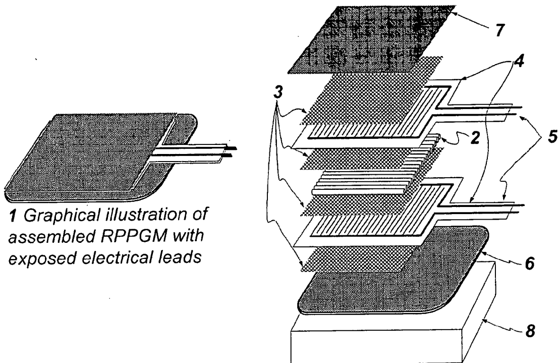
9 Breakout of part assembled in single lamination step, possibly on a non-flat surface
