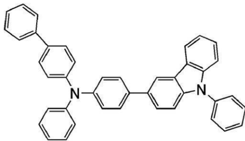
PCBA1BP
