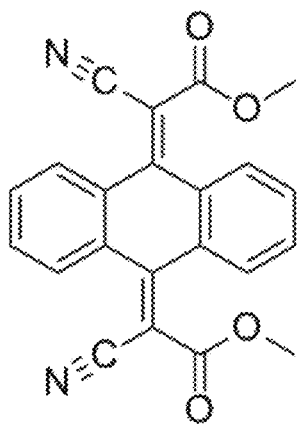
Formula IIIdi
