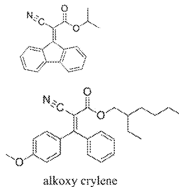
Formula IIai
