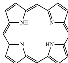
Structure of porphine, the simplest porphyrin
