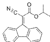
Formula IIai
