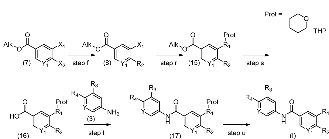
Reaction Scheme V:
