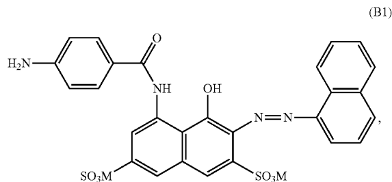
a compound of formula (B1)
