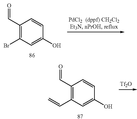
Scheme 10. Synthesis of rigid analogues (amine)
