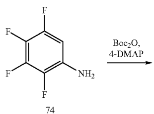
Scheme 8. Synthesis of tetrafluoroquinazolinone
