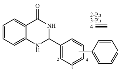
Phenyl Analogues/Isosteres
