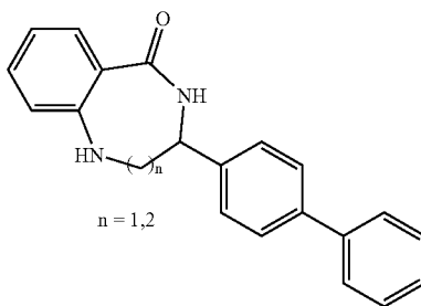
Ring Expansion
