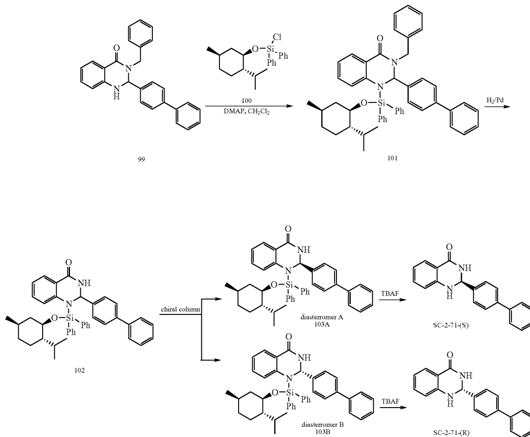
Scheme 12. Chiral resolution of SC-2-71.
