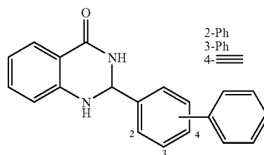
Phenyl Analogues/Isosteres
