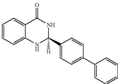
Chiral Analogue
